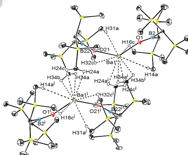
Figure 3. Representation of the molecular structure of [Ba(OB[CH(\text{SiMe}_3)_2]_2)_2] ( 2 ), showing the pattern of eight Ba\cdots H_3C intra- and intermolecular interactions in dotted lines. H atoms other than those interacting with Ba are omitted for clarity. Only the main component of the disordered \text{SiMe}_3 fragment is depicted. Pertaining Ba\text{--}H interatomic distances (Å): Ba1\text{--}H14A = 3.119(3) , Ba1\text{--}H16C
