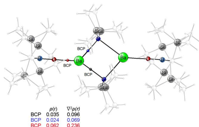
Figure 4. Topological QTAIM parameter (electron density \rho(r) in eÅ -3 and its Laplacian \nabla^2\rho(r) in eÅ -5 ) of crucial bond critical points (BCP) located for [Ba{ \mu^2 -N(SiMe 3 ) 2 }{OB[CH(SiMe 3 ) 2 ] 2 }] 2 ( 3 ).
