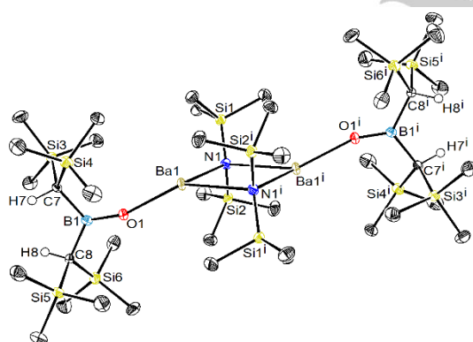
Figure 1. ORTEP representation of [Ba\{\mu^2\text{--}N(\text{SiMe}_3)_2\}(OB[CH(\text{SiMe}_3)_2]_2)_2] ( 3 ). Ellipsoids at the 50% probability level. H atoms (other than BCH) omitted for clarity. Selected bond lengths (Å) and angles ( ^\circ ): Ba1\text{--}O1 = 2.3999(14) , Ba1\text{--}N1 = 2.7210(16) , Ba1\text{--}N1' = 2.8912(17) , O1\text{--}B1 = 1.332(3) ; O1\text{--}Ba1\text{--}N1 = 121.64(5) , O1\text{--}Ba1\text{--}N1' = 144.18(5) , N1\text{--}Ba1\text{--}N1' = 82.34(5) , B1\text{--}O1\text{--}Ba1 = 160.00(14) , O1\text{--}B1\text{--}C8 = 123.38(18) , O1\text{--}B1\text{--}C7 = 120.05(18) , C8\text{--}B1\text{--}C7 = 116.57(17) .
