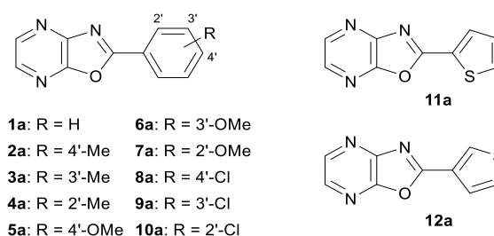
Figure 1. Starting 2-arylated oxazolo[4,5- b ]pyrazines.
