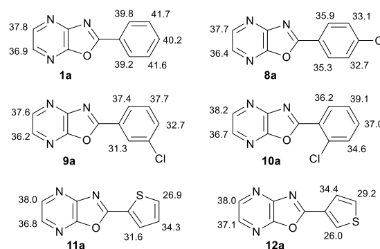
Figure 4. Calculated pK a (THF) values of 1a , 8a-10a , 11a and 12a .
