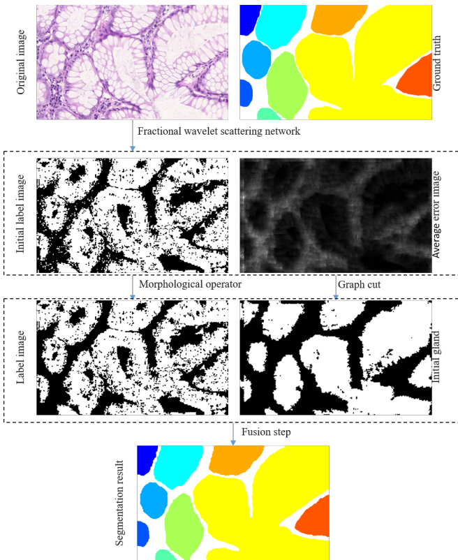
Fig. 5. The framework structure of the proposed gland segmentation algorithm.
