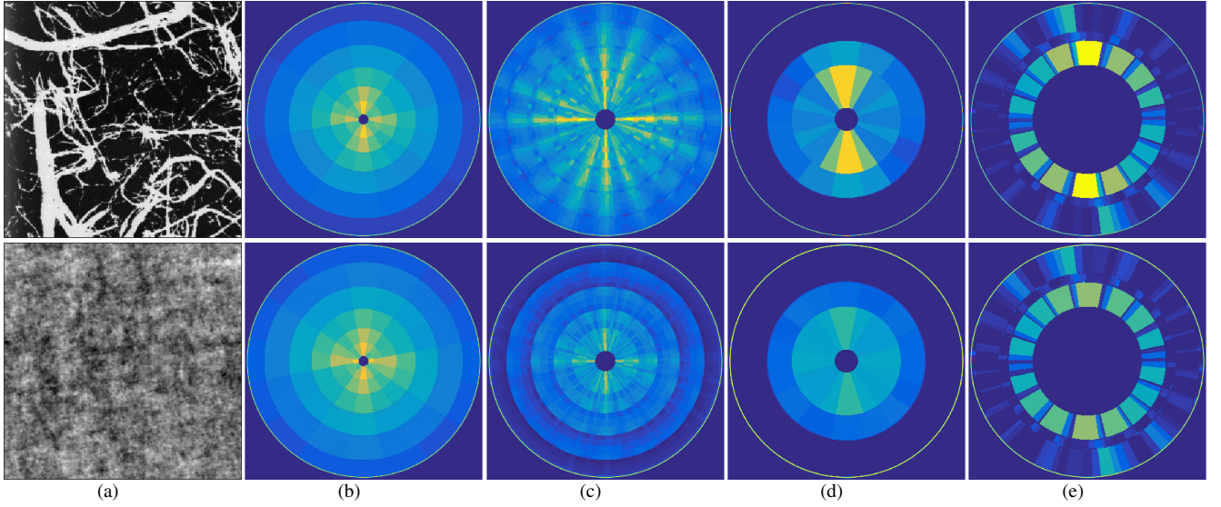
Fig. 1. (a) Realizations of two stationary processes X(\mu) . Top : Brodatz texture. Bottom : Gaussian process. (b) First-order scattering coefficients S[\lambda_1]x from the ScatNet [1] are nearly the same ( \alpha_1 = 1.00 , \alpha_2 = 1.00 ). (c) Second-order scattering coefficients S[\lambda_1, \lambda_2]x from the ScatNet [1] are clearly different ( \alpha_1 = 1.00 , \alpha_2 = 1.00 ). (d) First-order fractional scattering coefficients S[\lambda_1]x from the FrScatNet are clearly different ( \alpha_1 = 1.00 , \alpha_2 = 0.70 ). (e) Second-order fractional scattering coefficients S[\lambda_1, \lambda_2]x from FrScatNet are also clearly different ( \alpha_1 = 1.00 , \alpha_2 = 0.70 ).
