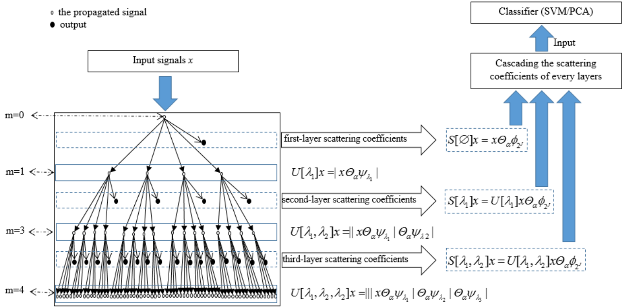
Fig. 2. An illustration of classification application of the FrScatNet.
