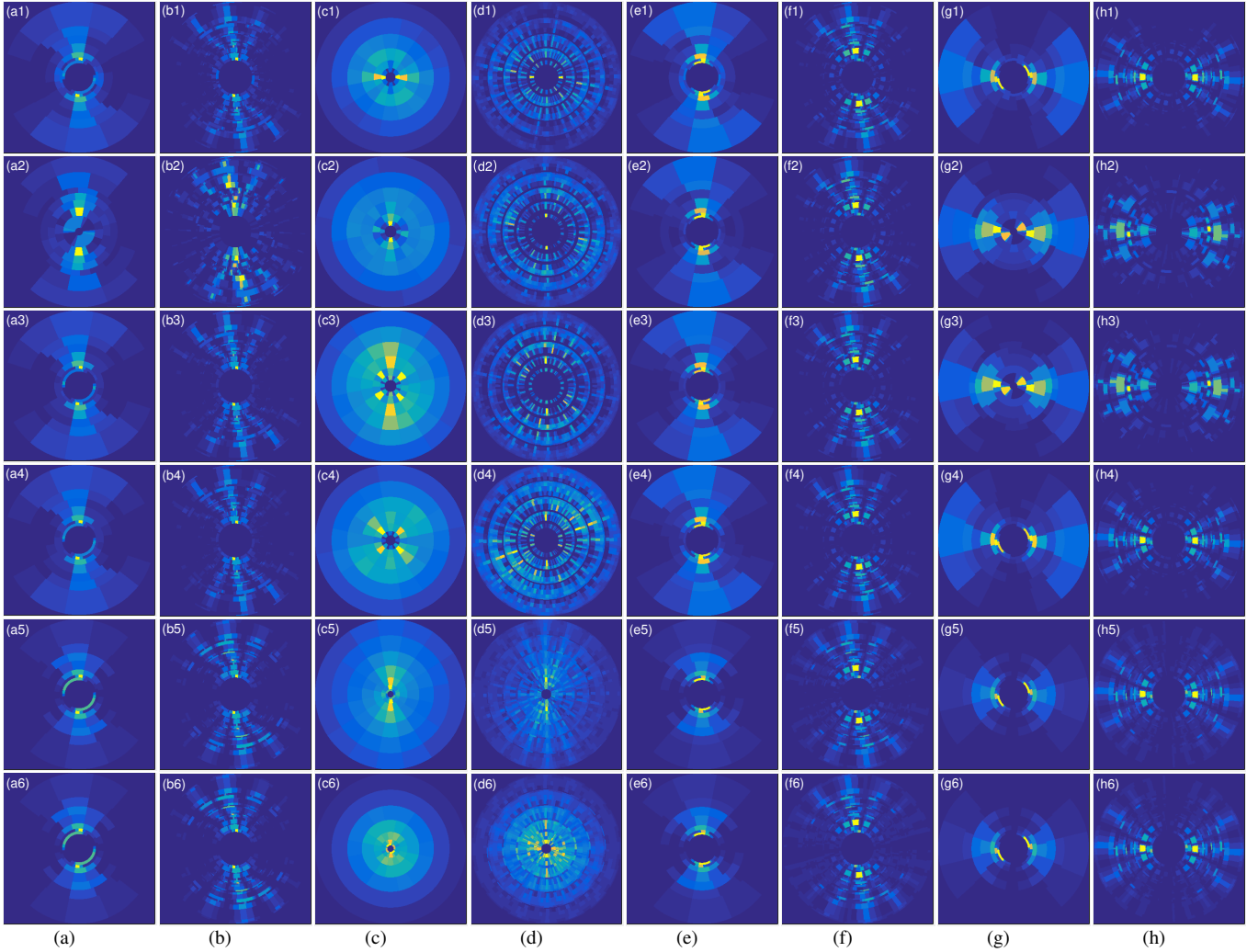
Fig. 4. Fractional scattering coefficients of two-dimensional images from the FrameworkI in different fractional orders. (a1-h1) are of a random benign image from the DB. (a2-h2) are of a random background image from the DB. (a3-h3) are from a random malignant image from the MB. (a4-h4) are from a random background image from the MB. (a5-h5) are computed from a random image in T01_bark1 of TSD. (a6-h6) are computed from a random image in T08_granite of TSD; (a) are first-order fractional scattering coefficients when \alpha_1 = 1.00, \alpha_2 = 0.40 . (b) are second-order fractional scattering coefficients when \alpha_1 = 1.00, \alpha_2 = 0.40 . (c) are first-order scattering coefficients when \alpha_1 = 1.00, \alpha_2 = 1.00 . (d) are second-order scattering coefficients when \alpha_1 = 1.00, \alpha_2 = 1.00 . (e) are first-order fractional scattering coefficients when \alpha_1 = 1.00, \alpha_2 = 1.60 . (f) are second-order fractional scattering coefficients when \alpha_1 = 1.00, \alpha_2 = 1.60 . (g) are first-order fractional scattering coefficients when \alpha_1 = 1.60, \alpha_2 = 1.00 . (h) are second-order fractional scattering coefficients when \alpha_1 = 1.60, \alpha_2 = 1.00 .
