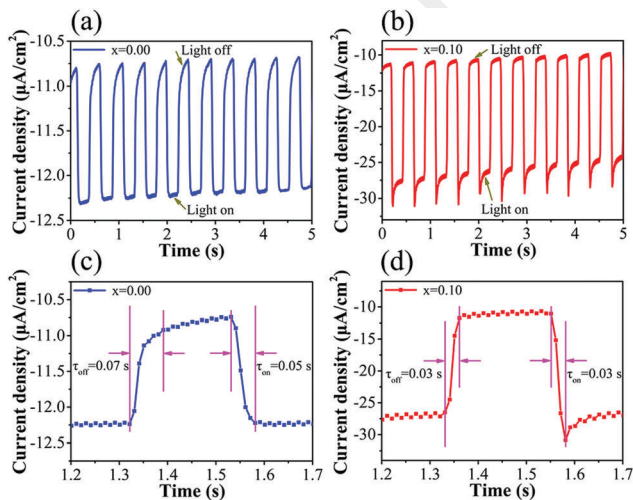
Fig. 6 Time-resolved PEC photoresponse by using \text{Sb}_2\text{Se}_3 (a) and (\text{Sn}_{0.10}\text{Sb}_{0.90})_2\text{Se}_3 (b) as the working electrode, respectively. (c) Magnified plot of one response cycle in (a), and (d) one response cycle in (b), used to obtain the response time and the recovery time.
