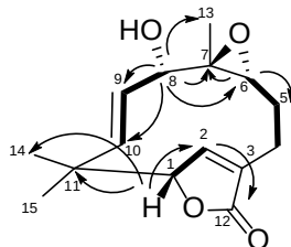
Fig. 2. Selected COSY (bold bond) and HMBC (H→C) correlations for compound 1 .
