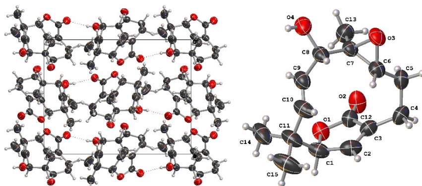
Fig. 3. Crystal packing and X ray structure for compound 1.
