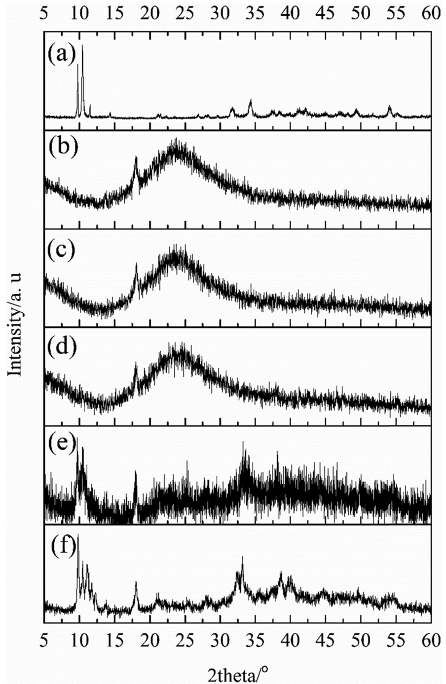
Fig. 8. XRD patterns of the starting TBH (a), \{\text{Ta}_6\text{Br}_{12}\}@ \text{SiO}_2 nanoparticles synthesized with C_{\text{TBH}} = 10 , R = 0.37 (b), C_{\text{TBH}} = 20 , R = 0.37 (c), C_{\text{TBH}} = 30 , R = 0.37 (d), C_{\text{TBH}} = 40 , R = 0.37 (e), and C_{\text{TBH}} = 30 , R = 0 (f); all these samples were washed for 10 times with water.
