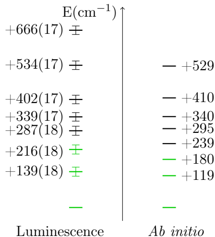
Figure S6: Representation of the energy splitting pattern of the {}^6H_{15/2} multiplet of Dy(III), according to the luminescence spectrum (left hand side) and the ab initio data (right hand side).
