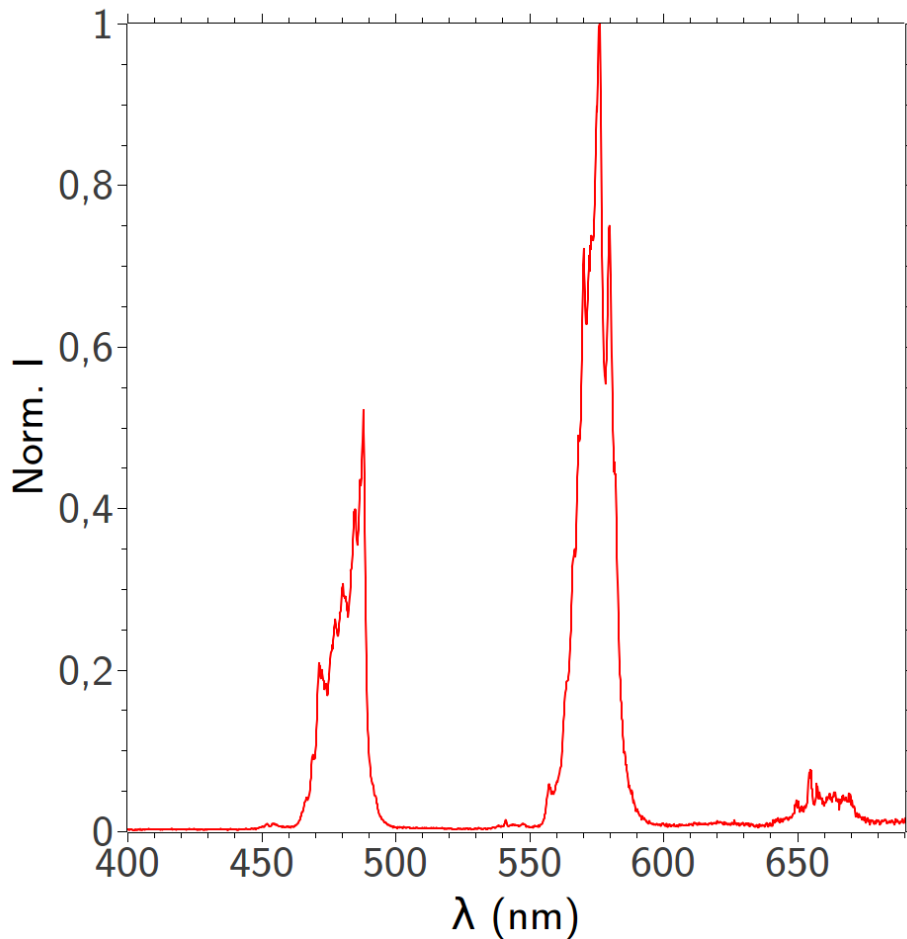
Figure S2: Room temperature solid state luminescence spectrum of [DyTp 2 Acac] ( \lambda_{ex} = 350 nm).
