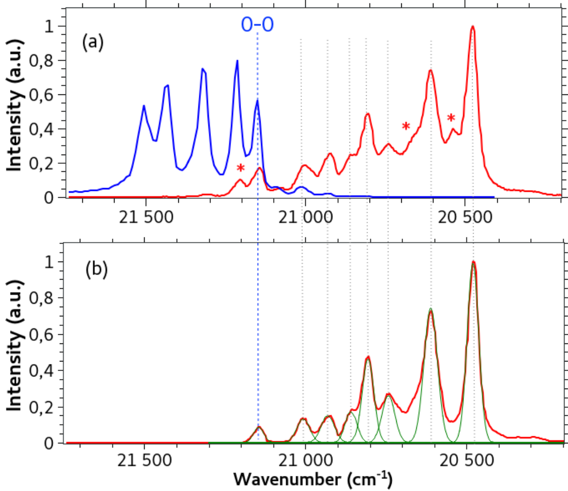
Figure S3: (a) Solid state emission (red) and excitation (blue) spectra of [\text{DyTp}_2\text{Acac}] , measured at 77 K. Hot bands are denoted by asterisks. (b) Solid state emission at 10 K. The dashed blue line depicts the (0,0) transition, and the solid green curves correspond to Gaussian fitting of the peaks.
