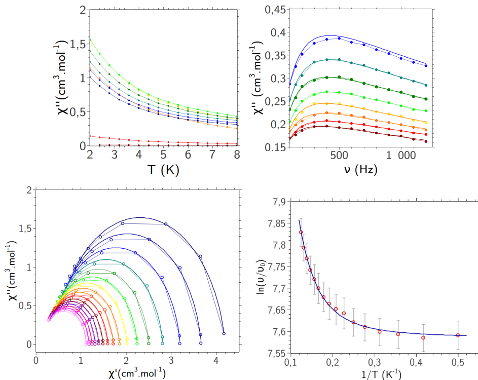
Figure S5: Upper left: \chi'' = f(T) curves for [DyTp 2 Acac], under a 0 Oe static field, for frequencies ranging between 1 Hz (brown) and 1400 Hz (blue). Upper right: \chi'' = f(\nu) curves for [DyTp 2 Acac], for temperature ranging between 2 K (blue) and 4.8 K (dark red). Solid lines correspond to the best fits. Lower left: Cole-Cole \chi'' = f(\chi') plot for temperatures ranging from 2 K (dark blue) to 8 K (purple). Solid curves correspond to the best fits. Lower right: \ln \nu = f(1/T) (Arrhenius) plot corresponding to the fits of the \chi'' = f(\nu) curves, with error bars (gray). The solid line corresponds to \nu = 1971(4) + 1.06(2)T^3 (best fit of the \nu = f(T) data).
