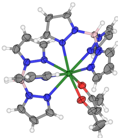
Figure S1: ORTEP drawing of the [\text{DyTp}_2\text{Acac}] complex (ellipsoids drawn at 50% probability). Colour scheme: blue, N; gray, C; green, Dy; pink, B; red, O; white, H.
