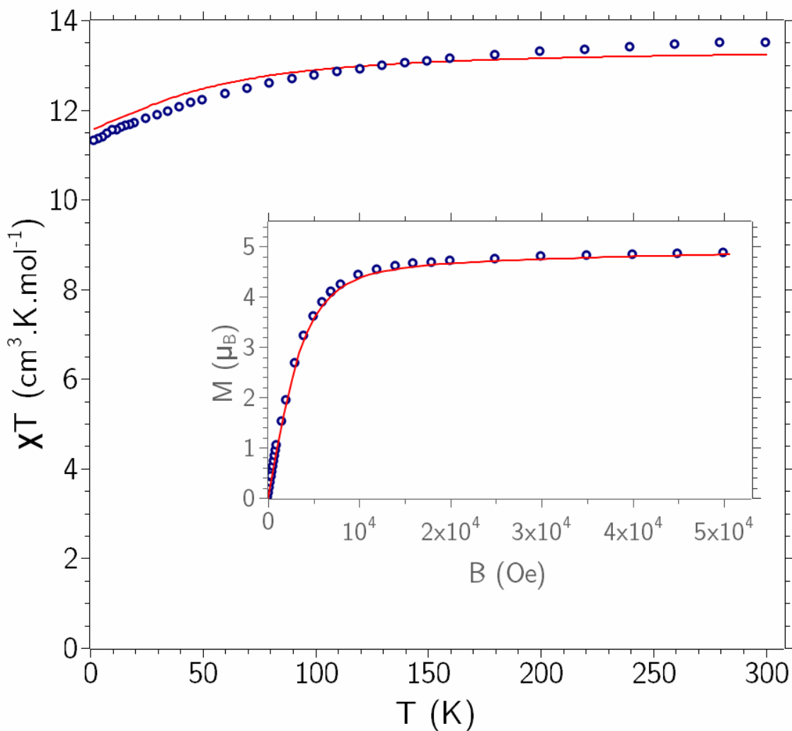
Figure S4: Main figure: Thermal dependence of the \chi T product for [\text{DyTp}_2\text{Acac}] , measured under a static field of 1000 Oe between 2 K and 300 K, on a powder sample (crushed single crystals). Inset: magnetic field dependence of magnetisation at 2 K, between 0 Oe and 50000 Oe. Solid red lines correspond to the ab initio model (—, vide infra ), and bullet points to the experimental data ( \circ ).
