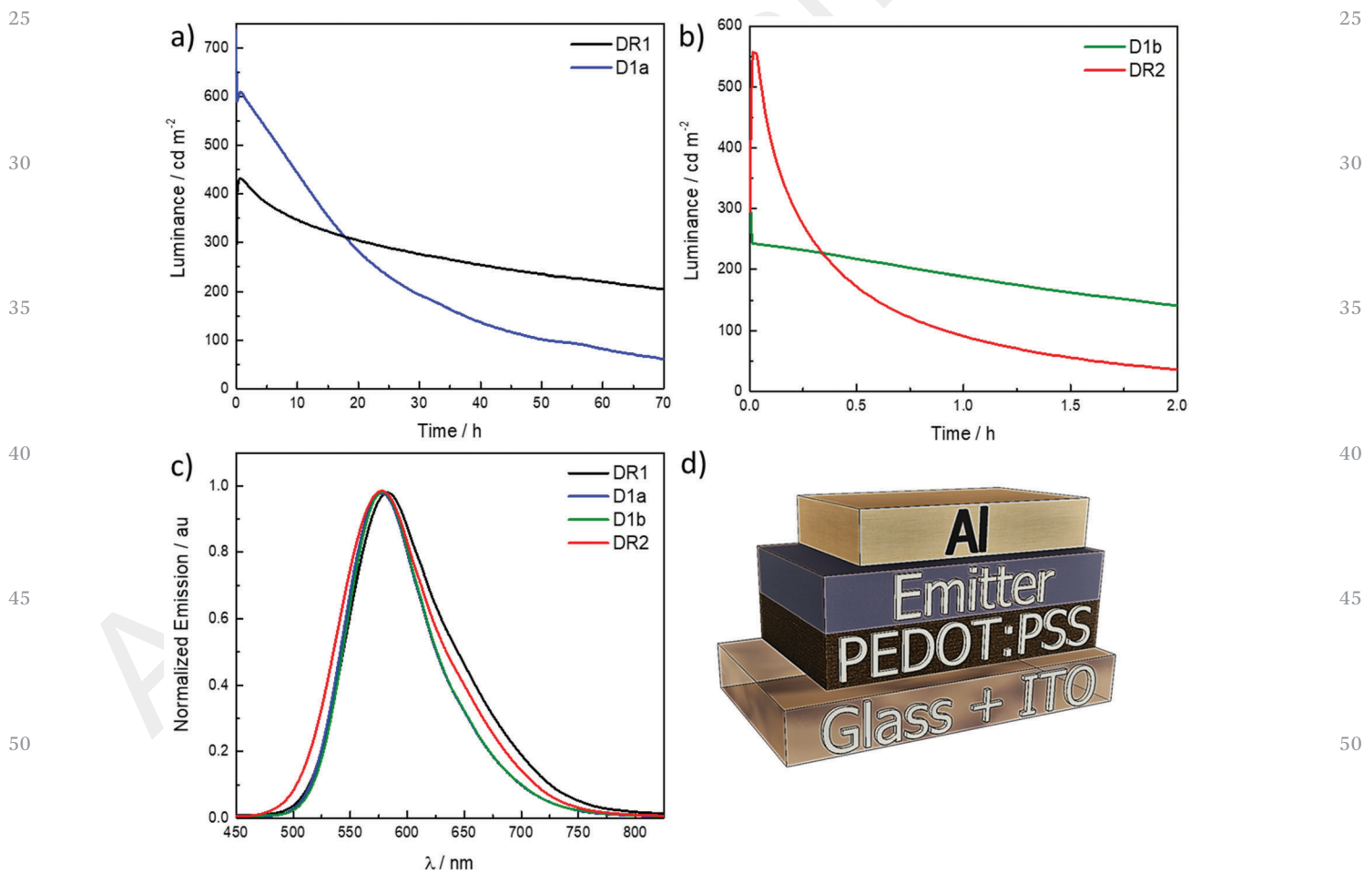
55 Fig. 6 Luminance versus time ( DR1 and D1a in (a) and D1b and DR2 in (b)) operated with a pulsed current of 100 \text{ A m}^{-2} (1 kHz, 50% duty cycle and block wave). (c) Electroluminescence spectrum. (d) LEEC architecture.
