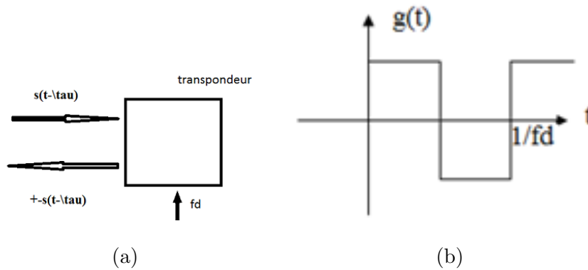
Figure 15. Modeling the behavior of the non-linear transponder.
