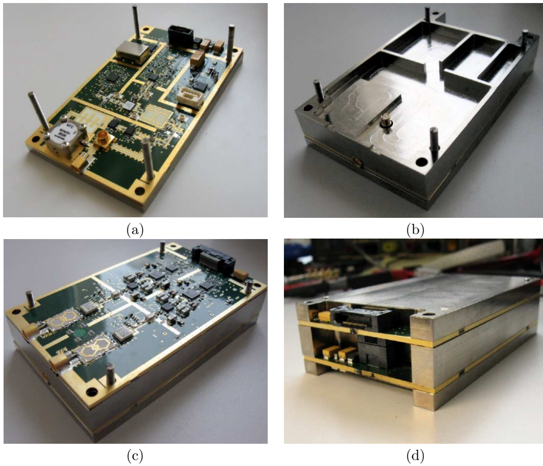
Figure 10. Radio module with transmission and receiving boards.
