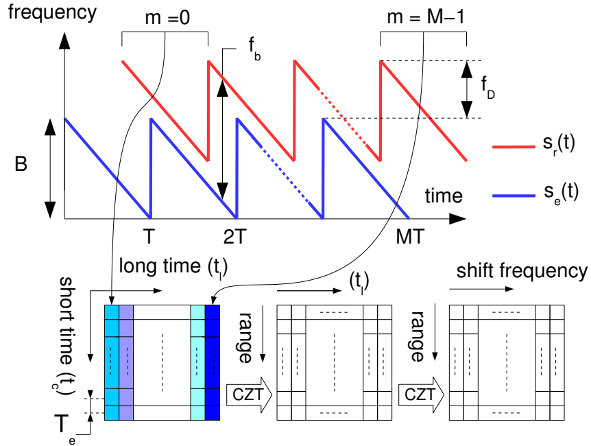
Figure 8. Instantaneous frequency over M transmitted ramps
