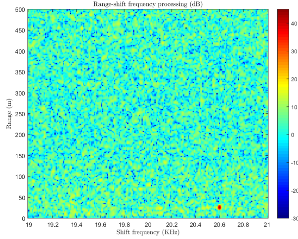
Figure 14. Range-shift frequency cartography established for a single target at distance R = 25 m from the radar with a transponder shift frequency f_D = 20.6 kHz.
