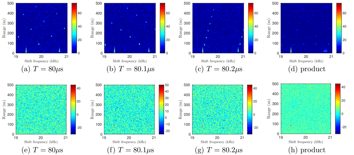
Figure 20. Range-shift frequency cartography provided from real measurements for two configurations of distance R = 12.5 m (first row) and R = 85 m (second row) and with different modulation times T = \{80, 80.1, 80.2\} \mu s . The figure (d) is the product of range-shift frequency cartographies given by (a), (b) and (c). The figure (h) is the product of range-shift frequency cartographies given by (e), (f) and (g).
