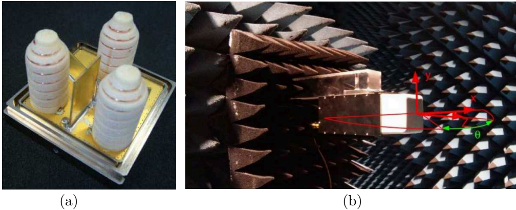
Figure 11. The realized compact antenna device with three radiating elements (a) and the front radiation patterns measured in an anechoic chamber, as a function of the orientation angle \theta (b).
