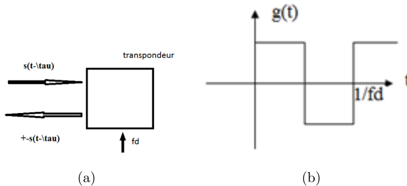
Figure 15. Modeling the behavior of the non-linear transponder.
