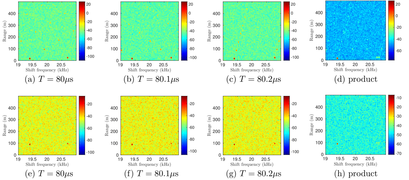
Figure 17. Simulations of range-shift frequency cartography with different modulation times T = [80, 80.1, 80.2]\mu\text{s} given respectively in (a), (b) and (c). The first and second rows are defined for a distance R = 12.5 m and R = 85 m between transponder and reader, respectively.
