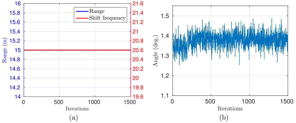
Figure 12. Range and shift frequency indoor measurements (a) and orientation angle indoor measurement curves (b).
