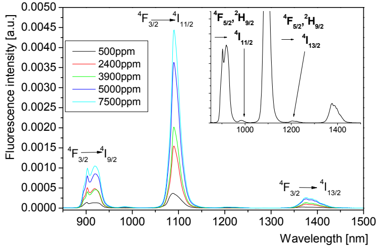
Fig. 9. Emission spectra of Nd 3+ doped 2S2G glass with different concentrations of rare earth.
