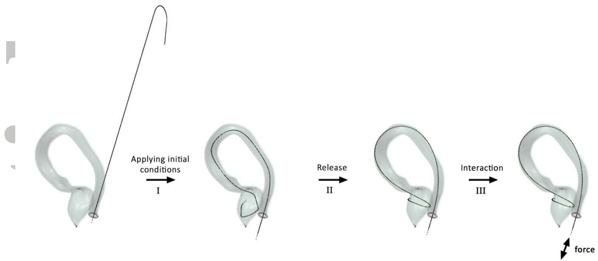
Fig.3 – Illustration of the simulation stages. After applying initial conditions, the guidewire was constrained on the centerline. After the constraints were relaxed, the guidewire reached its final equilibrium. Then insertion force could be varied.
