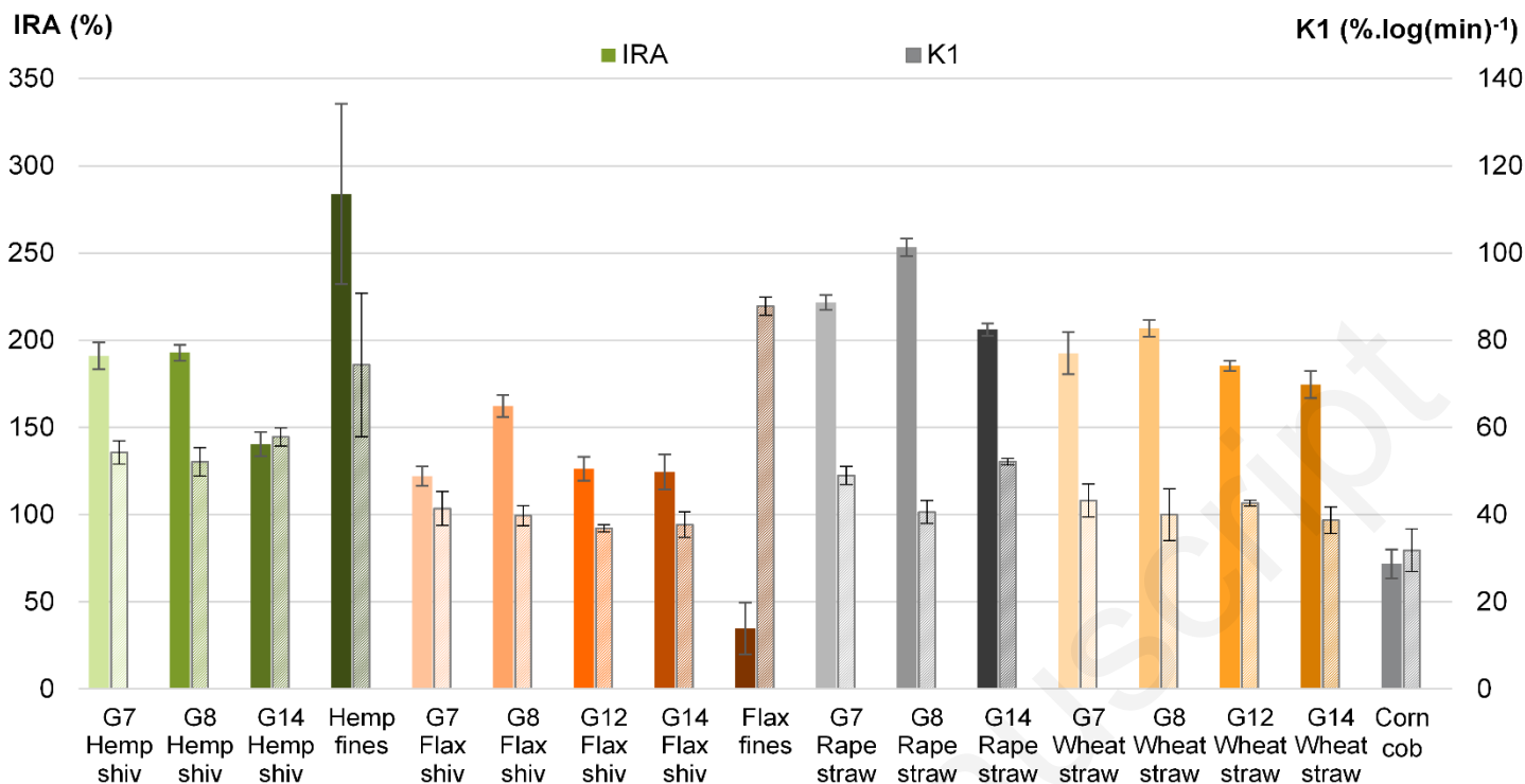
Figure 28: Water absorption, average values and standard deviations of fitting curve parameters IRA and K1
