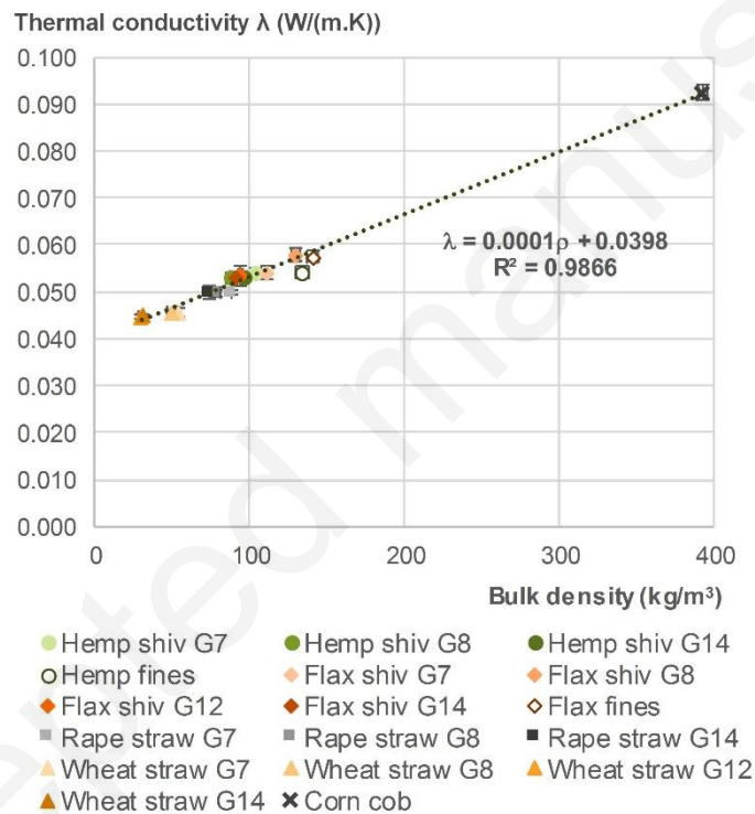
Figure 34: Thermal conductivity versus bulk density at (23°C, dry state)
