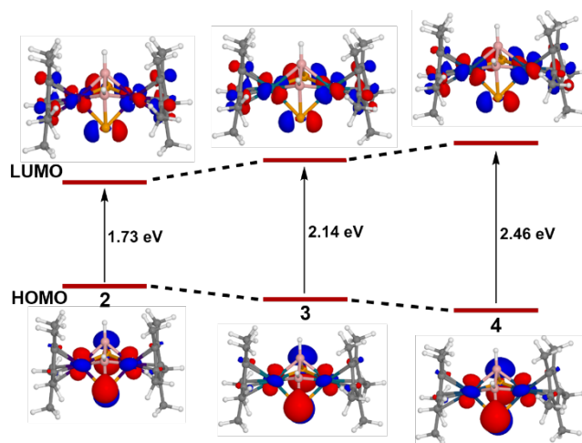
Figure 2. Frontier molecular orbital diagram of 2-4 (contour value: ±0.05 [e/bohr 3 ] 1/2 ).
