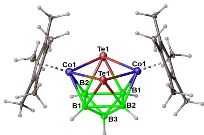
Figure 3. Molecular structure of 5 . Selected bond lengths (Å) and angles (°): Co1-Te1 2.5019(6), Te1-B1 2.347(5), Te1-B2 2.347(5), Co1-B1 2.154(5), Co1-B2 2.149(5), B1-B2 1.824(8), B2-B1 2.015(6), B1-B3 1.680(6), B3-B2 1.680(6), B(1)-Co(1)-Te(1) 94.42(14), B(1)-Te(1)-B(2) 50.85(16), B(1)-B(3)-B(2) 73.7(3).
