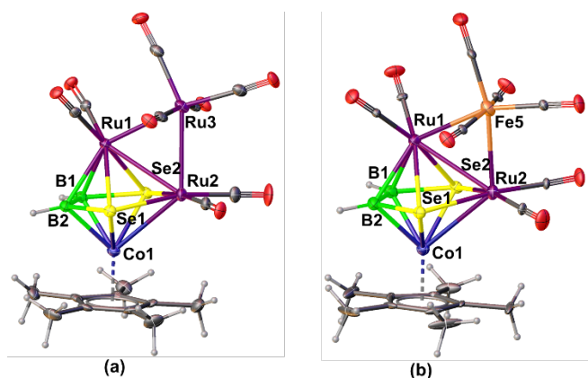
Figure 5. Molecular structures of 7 and 12 . Selected bond lengths ( \text{\AA} ) and angles ( ^\circ ): (a) Ru1-Ru2 2.911(5) , Ru1-Ru3 2.776(5) , Co1-B1 2.151(5) , Co1-Se1 2.4143(7) , Ru2-Se2 2.526(6) , Ru1-B1 2.299(5) , Se2-B1 2.032(5) , B1-B2 1.673(7) , B2-B1-Se2 116.9(3) , Ru1-Ru3-Ru2 63.423(12) ; (b): Ru1-Fe5 2.7198(8) , Ru2-Fe5 2.6739(9) , Co1-B1 2.152(6) , Co1-Se1 2.3966(7) , Co1-Se2 2.4058(8) , Ru2-Se1 2.5183(6) , Ru1-B1 2.301(6) , Se2-B1 2.010(6) , B1-B2 1.647(9) ; B2-B1-Se2 117.9(4) , Ru1-Fe5-Ru2 64.63(2) .
