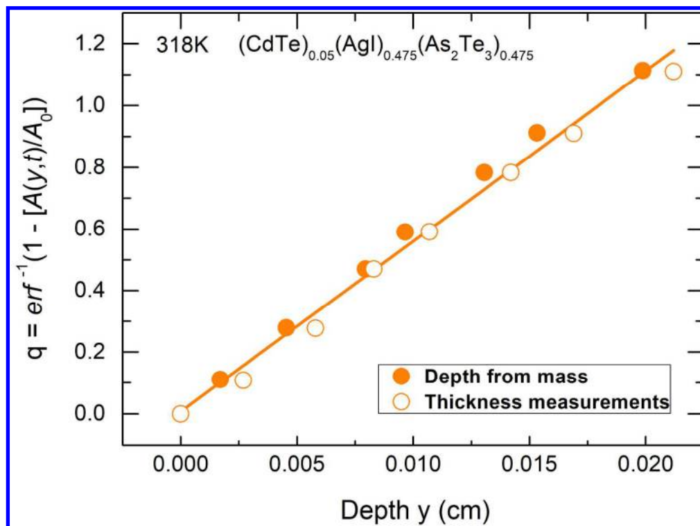
Figure 1. Typical ^{110\text{m}}\text{Ag} tracer diffusion profile for a (\text{CdTe})_{0.05}(\text{AgI})_{0.475}(\text{As}_2\text{Te}_3)_{0.475} glass annealed at 45 °C for 17 days. The penetration depth was calculated using (a) weight changes (filled circles) and (b) direct thickness measurements (open circles). The solid line shows a least-square fit of all experimental data points (open and filled circles) to Equation (2) where q = \text{erf}^{-1}(1 - A(y,t)/A_0) .
