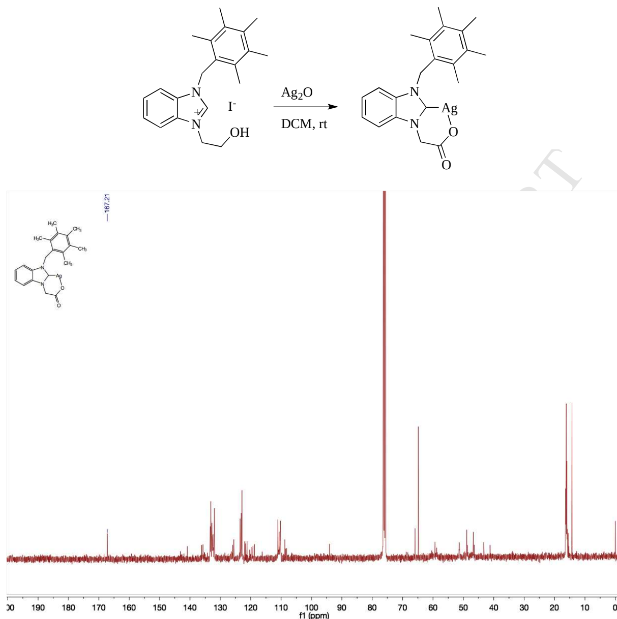
Figure 3. Proposed structure of in situ synthesised Ag(I)-NHC complex and 13 C NMR spectra. To synthesis complex 6 , 0.5 mmol RuCl 2 (HMB) 2 was added to the DCM solution of Ag(I)-NHC in dark. After stirring 24 h at room temperature, reaction mixture was filtrated upon celite and all volatiles removed under high vacuum. By dissolving the crude product of 6 in DCM/diethyl ether solution led to obtain single crystals suitable for X ray diffractions analysis. The 1 H NMR of 6 in CDCl 3 confirms the formation of chelated Ru(II)-NHC complexes by evanescent NCHN proton. C 2 carbon of chelated Ru(II)-NHC complexes in 13 C NMR spectra shifted to 191.5 ppm, also confirm formation of 6 . Also, CH 2 COO-Ru carbon
