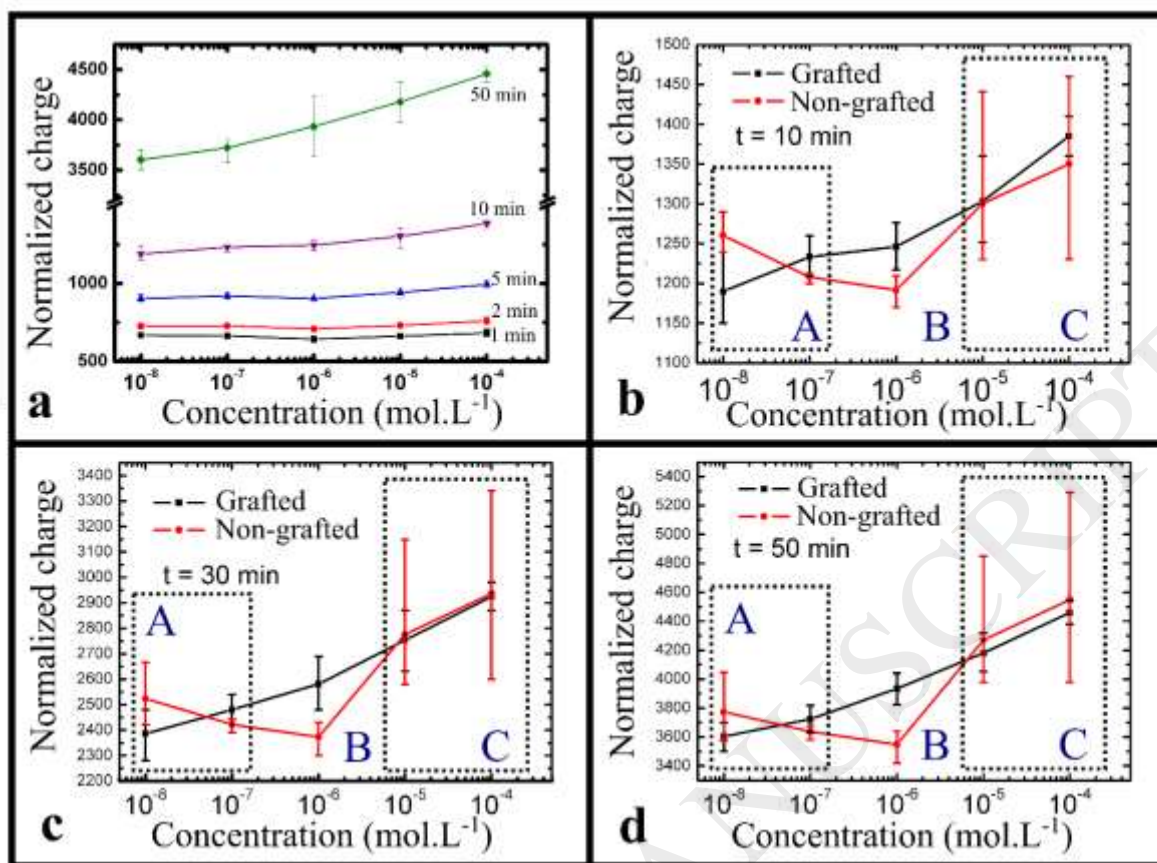
Fig. 8 Normalized charge measurement for different \text{Pb}^{2+} concentrations (a) and exposure times (1, 2, 5, 10 and 50 min). Normalized charge comparison between grafted and non-grafted poly-Si nanoribbons based devices after 10 min (b), 30 min (c) and 50 min (d) exposure.
