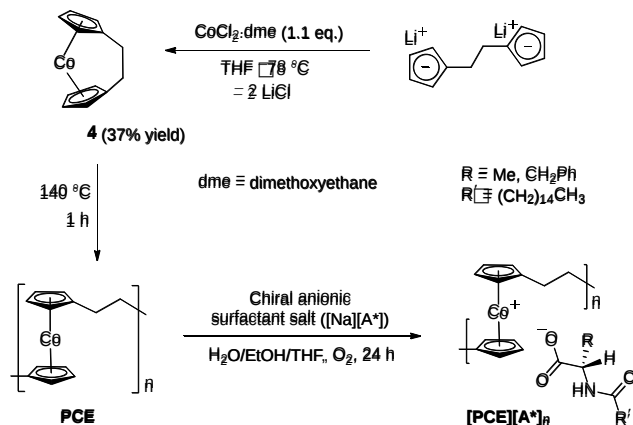
Scheme 1. Synthesis and thermal ring-opening polymerization of dicarba[2]cobaltocenophane 4 , followed by oxidation in the presence of chiral anionic surfactants to yield [PCE][A*] n complexes.
