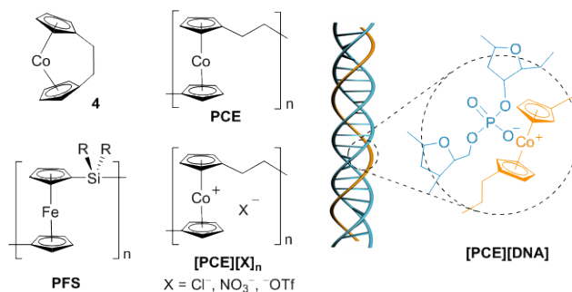
Figure 2. Structures of dicarba[2]cobaltocenophane 4 , poly(cobaltocenylethylene) (PCE), poly(cobaltoceniumethylene) ( [PCE][X]_n ), polyferrocenylsilane (PFS) and [PCE][DNA] bioconjugate.
