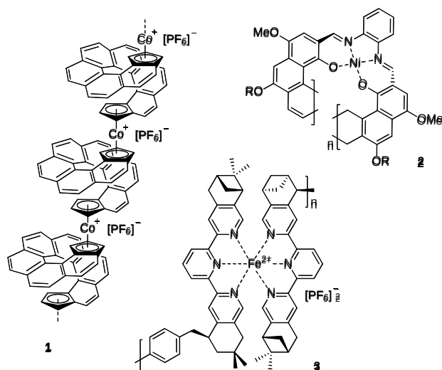
Figure 1. Metal-containing chiral oligomers and coordination polymers 1–3.
