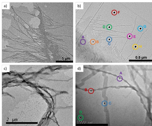
Figure 7. TEM images obtained after drop-casting an aliquot of solutions of [PCE][C_{16}\text{-L-Ala}]_n complex in a) ethanol (ca. 12 mg mL -1 ) and b) spot EDX analyses of film and fibrous material (drop cast from 12 mg mL -1 ethanolic solution), or c) by drop-casting suspensions of [PCE][C_{16}\text{-L-Ala}]_n assemblies in water, and d) spot EDX analyses of helices. For detailed EDX analysis of spots see Supporting Information (Figs. S9 and S28).
