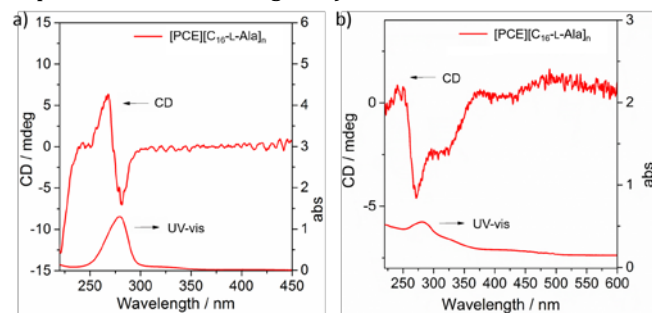
Figure 8. a) Solution state CD and UV-vis spectra of [PCE][C_{16}\text{-L-Ala}]_n at 0.5 mg mL -1 in EtOH, and b) solid state CD and UV-vis spectra of the [PCE][C_{16}\text{-L-Ala}]_n self-assembly product formed in water.
