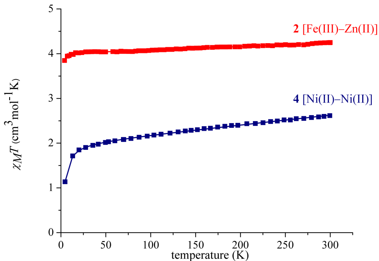
Figure 2. An overlay of variable temperature \chi_M T plot of powder sample of the hetero- and homodinuclear complexes ( 2 and 4 ) supported over symmetrical ligand supported over symmetrical ligand 1 measured at 5000 Oe (the solid line represents the best fit curve).
