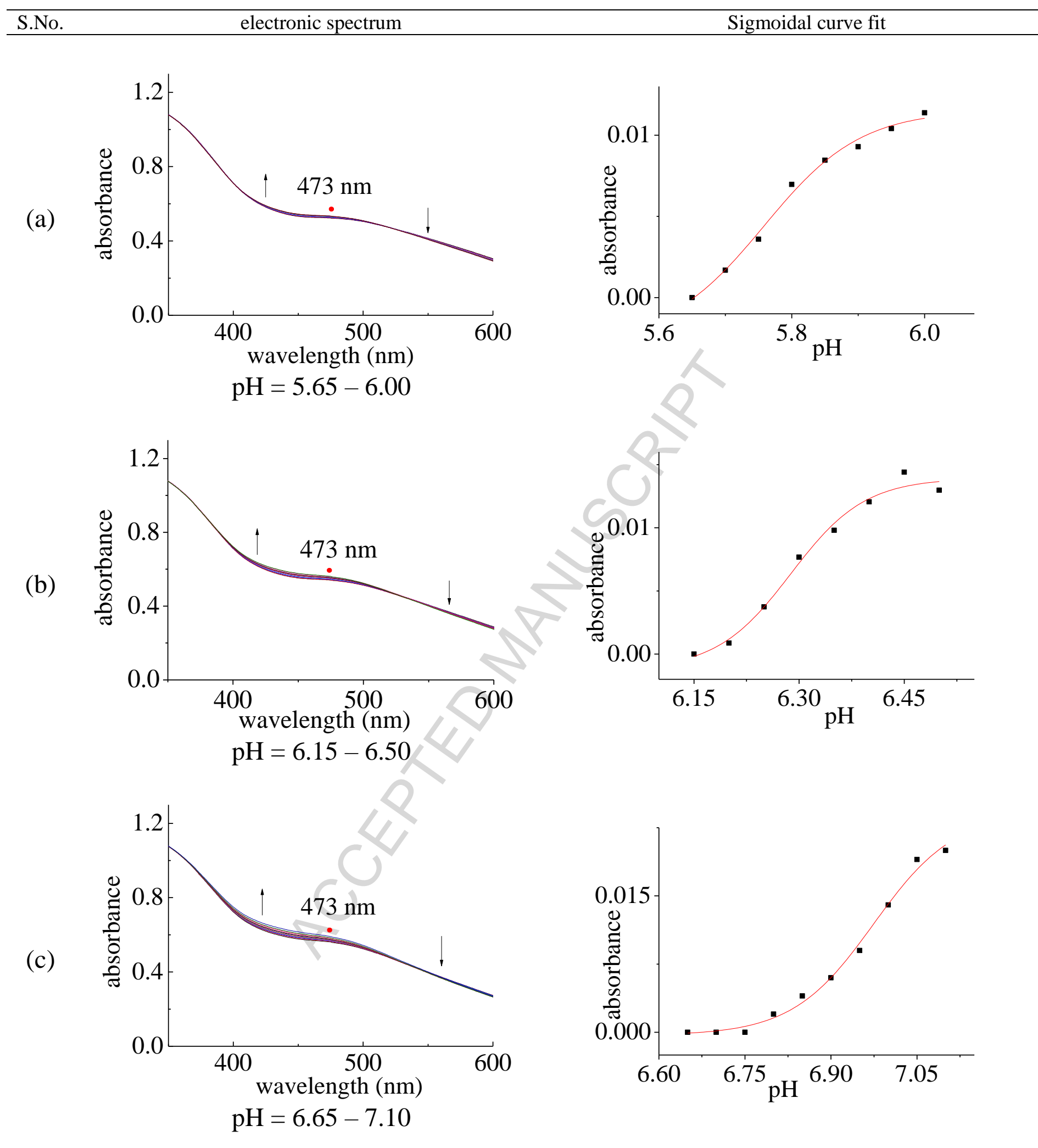
Figure 3. Electronic spectrum (Column 1) in different pH ranges [(a) 5.65 – 6.00, (b) 6.15 – 6.50, (c) 6.65 – 7.10] and the corresponding titration plot (Column 2) performed at 473 nm (LMCT band) as a function of pH with incremental additions of 0.1 M NaOH [5 \mu L] in an \text{CH}_3\text{CN}/\text{H}_2\text{O} ( v/v 1:1) solution of 2 ( 6.0 \times 10^{-4} M) containing I = 0.1 M (KCl).
