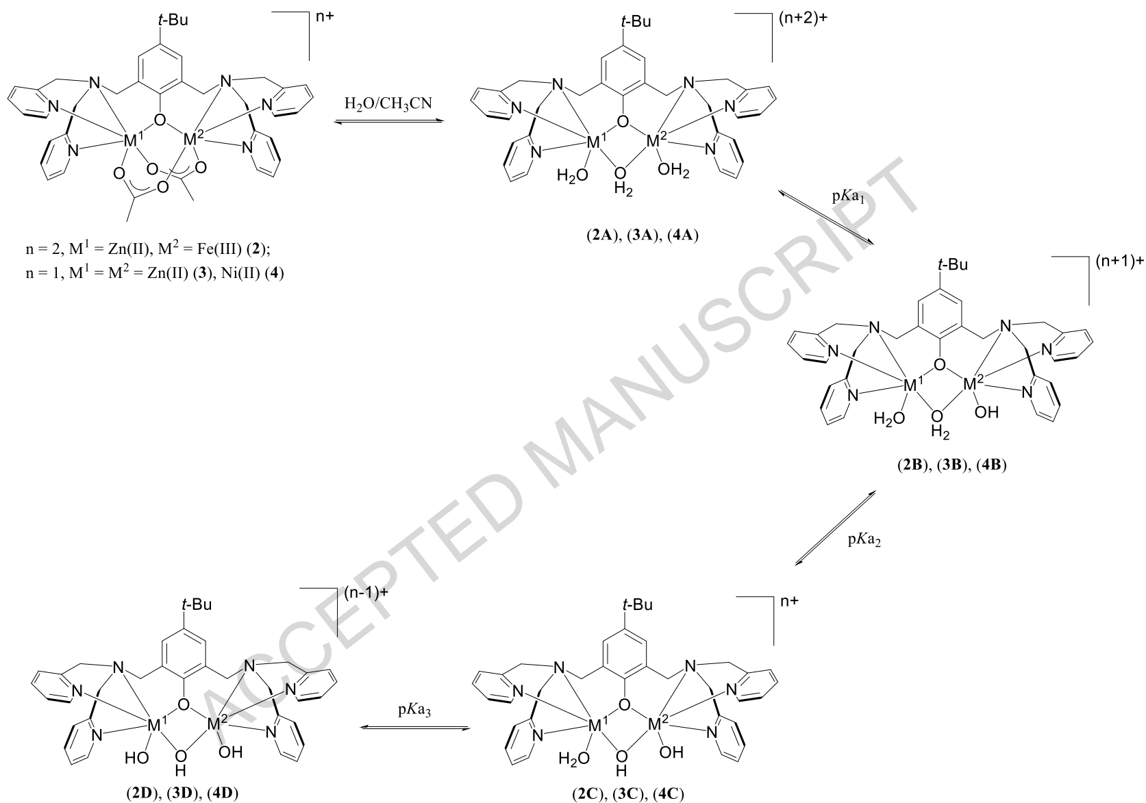
Scheme 2. Equilibrium of chemical species in \text{CH}_3\text{CN}/\text{H}_2\text{O} solution proposed for the hetero- and homodinuclear complexes ( 2–4 ) supported over symmetrical ligand 1 .
