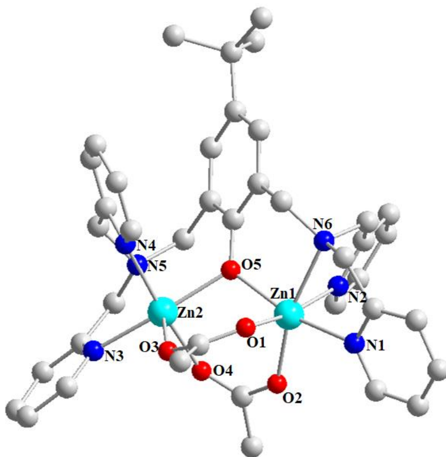
Figure 1. Perspective view of complex 3 with partial atom numbering schemes. A BPh 4 - anion has been omitted for the sake of clarity. Selected bond lengths (Å) and angles (°): Zn1–O2 2.005(4), Zn1–O5 2.034(3), Zn1–O1 2.112(4), Zn1–N1 2.157(4), Zn1–N2 2.193(4), Zn1–N6 2.251(5), Zn2–O3 2.026(4), Zn2–O5 2.040(3), Zn2–N3 2.125(4), Zn2–O4 2.150(4), Zn2–N4 2.204(5), Zn2–N5 2.207(4), Zn1–O5–Zn2 109.99(16).
