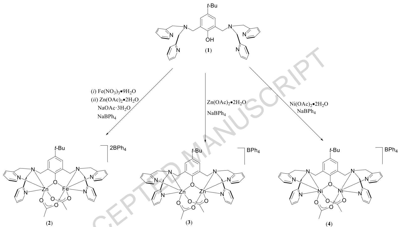
Scheme 1. Synthesis of the the hetero- and homodinuclear complexes supported over symmetrical [N 6 O] ligand 1 .
