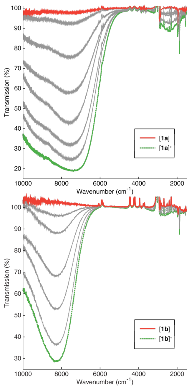
Figure 6. The reversible spectral changes observed upon spectroelectrochemical oxidation of 1a, b \rightarrow 1a, b + in the 1000 – 10000 cm -1 region.
