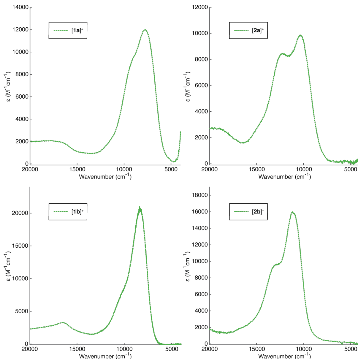
Figure 5. The spectroelectrochemically generated NIR spectra of [\mathbf{1a,b}]^+ and [\mathbf{2a,b}]^+ in \text{CH}_2\text{Cl}_2 / 0.1 M \text{NBu}_4[\text{PF}_6] at room temperature.
