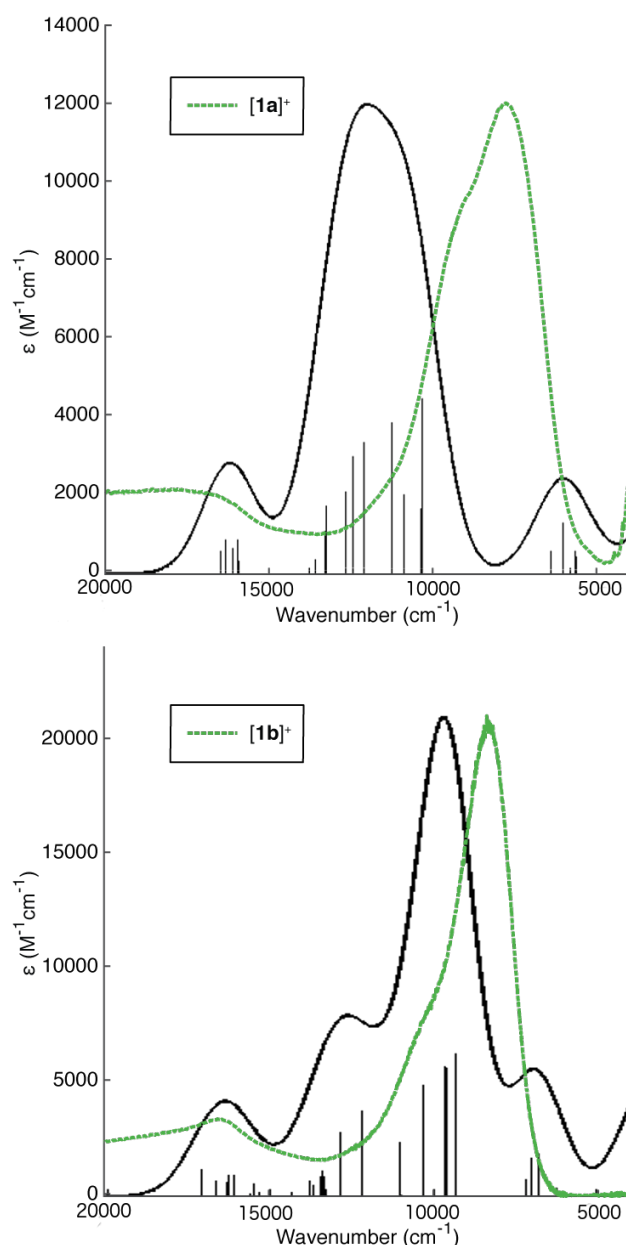
Figure 8. The spectroelectrochemically generated NIR spectra of [1a,b]^+ (green, dotted lines) and computed spectra, convoluting a simple average of the stick spectra of the various conformers (black, solid line, with stick spectra).
