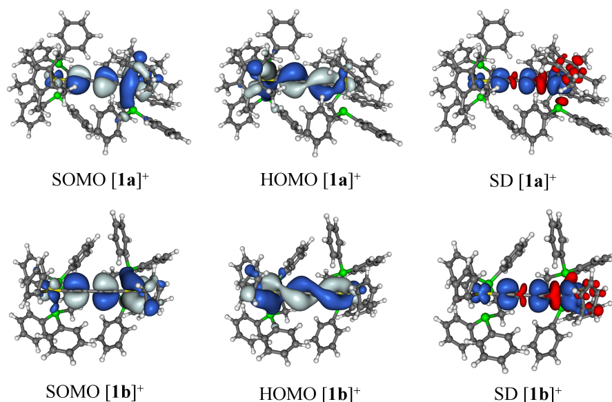
Figure 4. Frontier molecular orbital plots (isosurface: \pm 0.02 a.u.) and spin-density plots (isosurface: \pm 0.001 a.u.) for [1a]^+ ( \Omega = 55^\circ ) and [1b]^+ ( \Omega = 36^\circ ) using Lh-SsirPW92-D3/def2-SVP (red color in the spin density marks negative values). Plots of related orbitals and spin-density distributions for other minima are given in the Supporting Information
