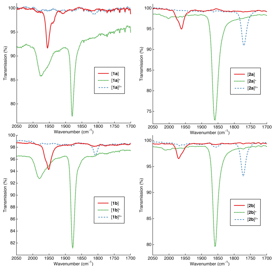
Figure 2. The \nu(\text{C}\equiv\text{C}) IR spectra of [\mathbf{1a}]^{n+} , [\mathbf{1b}]^{n+} , [\mathbf{2a}]^{n+} and [\mathbf{2b}]^{n+} ( n = 0, 1, 2 ) in 0.1M NBu 4 PF 6 / CH 2 Cl 2 .
