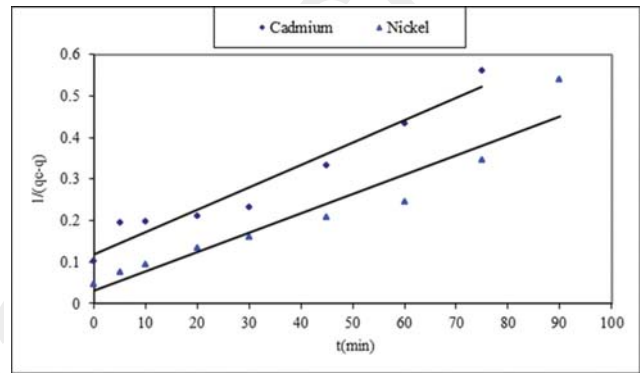
Fig. 6. Constant second-order speed of biosorption of the mixture \text{Cd}^{2+} and \text{Ni}^{2+} .
