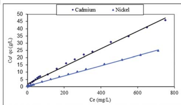
Fig. 18. Langmuir isotherm of the mixture \text{Ni}^{2+} and \text{Cd}^{2+} .
