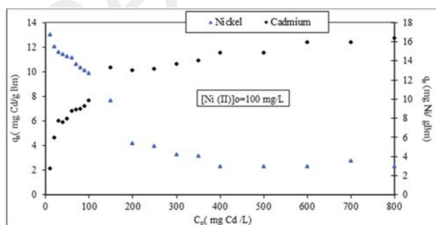
Fig. 16. Influence initial concentration in \text{Cd}^{2+} ions on the capacity of biosorption \text{Cd}^{2+} and \text{Ni}^{2+} of the treated biomass.
