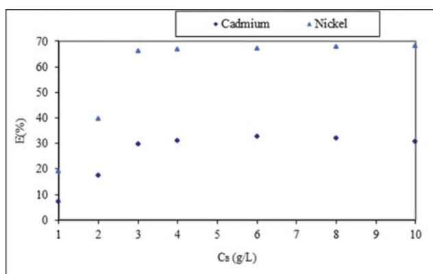
Fig. 15. The influence of the concentration of the biomass treated on the rate of biosorption of the mixture \text{Cd}^{2+} and \text{Ni}^{2+} .
