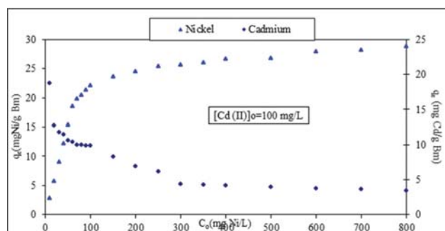
Fig. 17. Variation of the capacity of biosorption of \text{Cd}^{2+} and \text{Ni}^{2+} according to the initial concentrations of \text{Ni}^{2+} .
