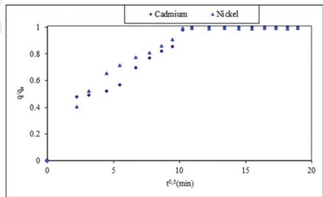
Fig. 9. Variation of q/q_e according to time.
