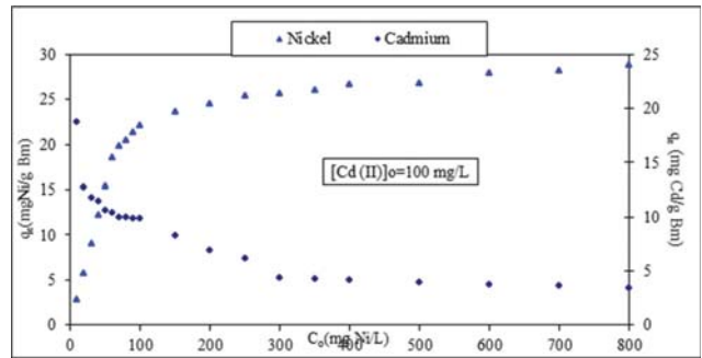
Fig. 17. Variation of the capacity of biosorption of Cd^{+2} and Ni^{+2} according to the initial concentrations of Ni^{+2} .
