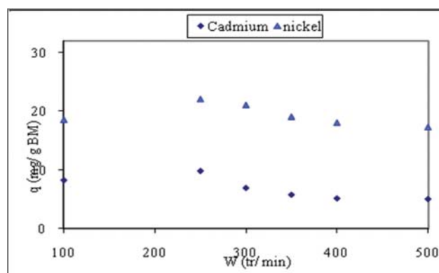
Fig. 14. The influence of the stirring velocity on the biosorption of Cd 2+ and Ni 2+ .
