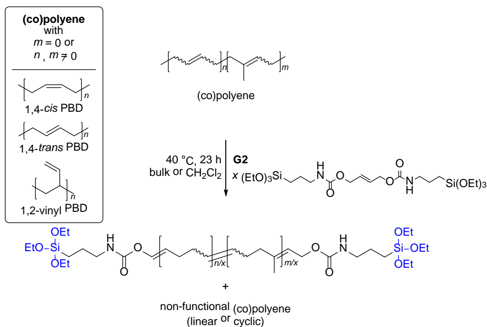
Scheme 16. Functional metathesis degradation reactions of PBDs ( m = 0 ) or P(BD-co-IP) ( n and m \neq 0 ) (co)polymers using G2 catalyst in the presence of a bis(triethoxysilyl)diurethane-based CTA towards the formation of bis(triethoxysilyl) telechelic polyenes. 73 Note that the
