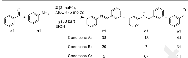
Scheme 2. Optimization of the procedure for reductive amination of benzaldehyde with aniline under the catalysis of manganese complex 2 . See main text for conditions definition and SI Table S4 for experimental details.
