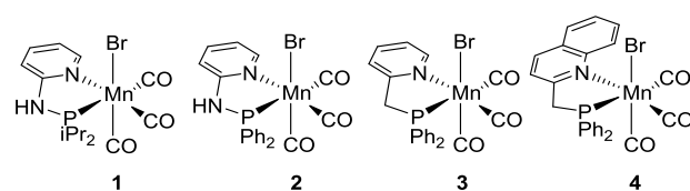
Scheme 1. Manganese complexes used in this study.
