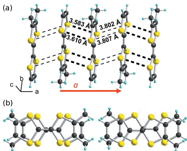
Figure 4 (a) A side view of one chain in (o\text{-Me}_2\text{TTF})_2\text{NO}_3 (stacking axis \mathbf{a} ) with intermolecular \text{S}\cdots\text{S} contacts shown as black dotted lines. (b) The two different overlap patterns within one chain: (left) eclipsed and (right) bond-over-ring.
