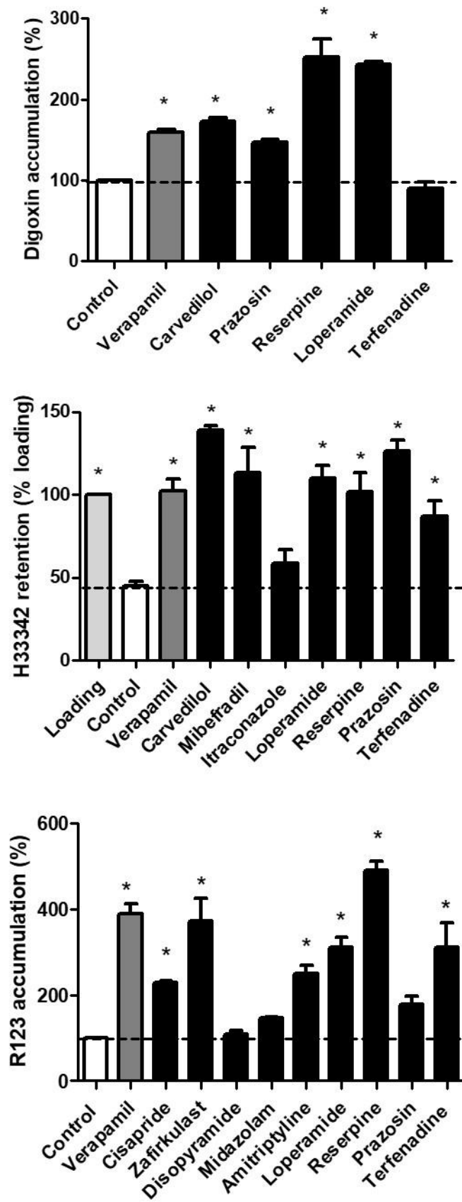
Fig. 2. Inhibitory effects of compounds on P-gp-mediated transport of digoxin, H33342 and Rh123. Accumulation of digoxin and Rh123 and retention of H33342 in P-gp-expressing MCF7R cells were determined in the absence (control)
