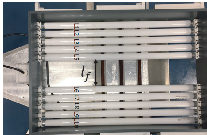
Figure 3. Global design of the antenna with agile plasma wall.
