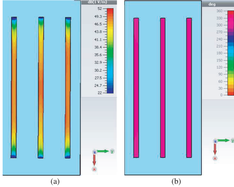
Figure 1. Electrical field distribution into the apertures. (a) Magnitude. (b) Phase.
