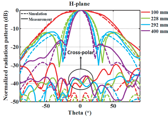
Figure 5. Normalized H -plane radiation patterns with the plasma wall.
