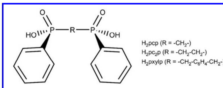
Chart 1. Molecular structure of a diphenyl-bisphosphinate with different substituting groups.
