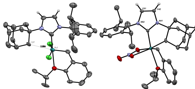
Figure 2. Solid-state structure of complex C1 (left) and complex Ru-2 (right) from single crystal X-ray diffraction. Displacement ellipsoids are drawn at 50% probability. Most hydrogen atoms have been omitted for clarity (N in blue, C in grey, Cl in green, O in red, H in white). For complex C1 : distance between C27 and Ru = 2.89 Å. For complex Ru-2 : distance between C27 and Ru = 2.06 Å.
