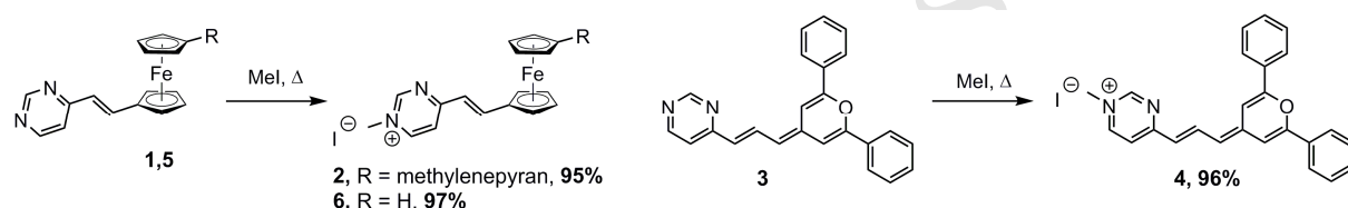
Scheme 2 Synthesis of N -methylpyrimidinium derivatives 2 , 4 and 6
