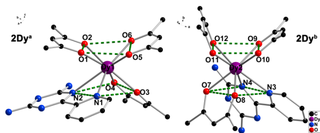
Figure 3. Molecular structures of 2Dy a (left) and 2Dy b (right). H atoms and solvent molecules are omitted for clarity.
