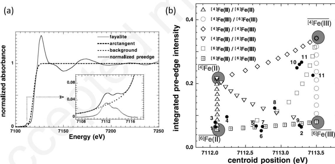
Figure 16: (a) The Fe K-edge absorption spectrum. The inset figure shows the pre-edge feature, which when normalized can be used to calculate the centroid position and integrated pre-edge intensity. (b) Comparison between pre-edge intensity and centroid position (eV) for different oxidation and coordination states of Fe in various Fe minerals. Black circles are 1 humite; 2 rhodonite no. 1; 3 rhodonite no. 2; 4 dumortierite; 5 potassian kaersutite; 6 kaersutite; 7 vesuvianite no. 1; 8 vesuvianite no. 2; 9 franklinite, 10 magnetite no. 1 & no. 2; 11 labradorite; 12 maghemite. Both (a) and (b) are reproduced with permission from Ref. 369. Copyright 2001 Mineralogical Society of America.
