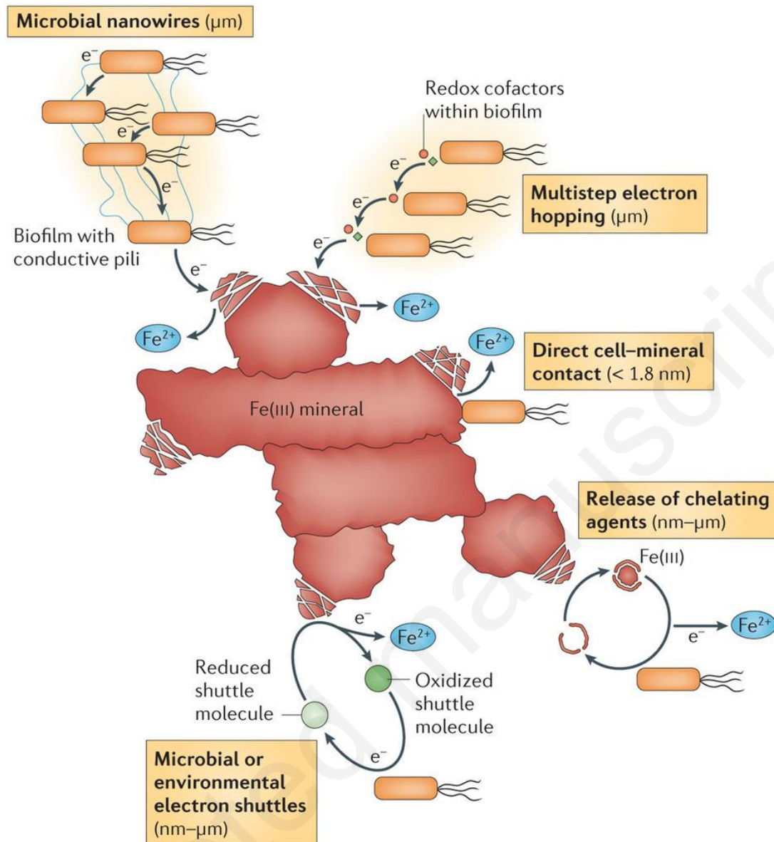
Figure 9: Possible electron transfer pathways during Fe(III) reduction. Direct contact between the Fe(III) minerals and the bacterial cell facilitates Fe(III) reduction over short distances. Bacteria secrete chelating agents or exploit microbial or environmental redox-active electron shuttles (such as flavins or dissolved and solid-state humic substances, respectively) to facilitate electron transfer over short (nm) and long ( \mu\text{m} ) distances. Electrically conductive pili and multistep electron hopping via redox cofactors that are present in biofilms have been implicated in long-distance extracellular electron transfer. Reproduced with permission from Ref. 232. Copyright 2014 Nature Publishing Group.
