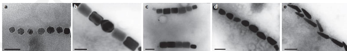
Figure 11: Different morphologies of magnetite produced by MTB's. Reproduced with permission from Ref. 294. Copyright 2016 Nature Publishing Group.
