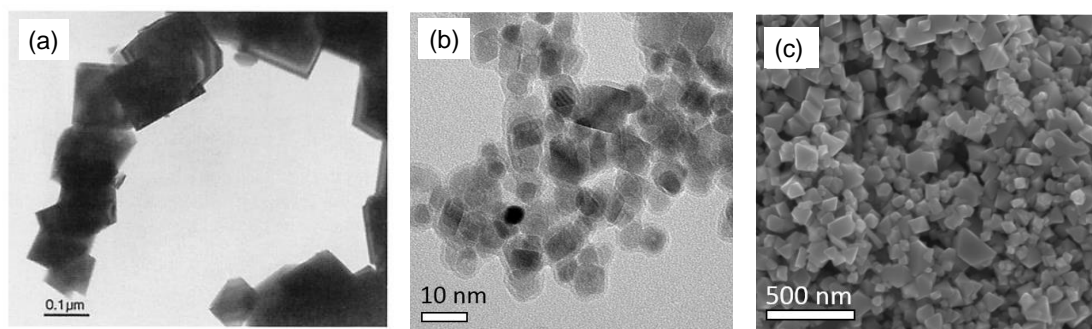
Figure 19: TEM images of magnetites synthesized by different procedures. (a) Magnetite synthesized by Schwertmann and Cornell 392 from \text{FeSO}_4 solution. Reproduced with permission from Ref. 392. Copyright 2000 John Wiley and Sons. (b) Nano-magnetite synthesized by Byrne et al. 48 from \text{FeSO}_4 solution by modifying method of Schwertmann and Cornell 392 , and (c) micro-magnetite synthesized by Byrne et al. 48 from \text{FeCl}_2 and \text{FeCl}_3 solution. Both (b) and (c) images are reproduced with permission from Ref. 48. Copyright 2016 Nature Publishing Group. TEM images of magnetite formed by abiotic transformation of ferrihydrite, lepidocrocite and goethite can be seen in Figure 8.
