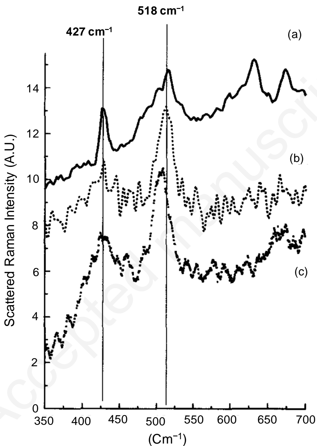
Figure 15: Microprobe Raman spectra of different green rusts (GRs): (a) natural GR, (b) synthetic \text{GR}(\text{CO}_3^{2-}) and (c) correspond to synthetic \text{GR}(\text{Cl}^-) . Reproduced with permission from Ref. 85. Copyright 1997 Elsevier.
