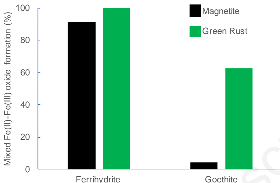
Figure 7: Transformation extent of ferrihydrite and goethite into mixed-valent iron minerals (magnetite and green rust) measured by Mössbauer Spectroscopy. Ferrihydrite and goethite were reacted with stoichiometric amounts of soluble Fe(II) and NaOH to form magnetite and green rust according to the reaction 3 and 4. Figure prepared by using the data reported in Table 2 of Ref. 51.
