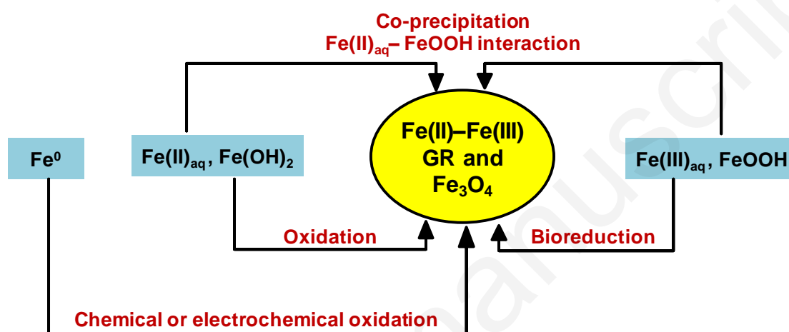
Figure 5: Overview of different pathways for the formation of magnetite (Fe 3 O 4 ) and green rust (GR).
