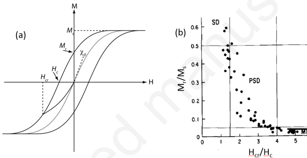
Figure 20: (a) A hysteresis loop shows how the magnetization ( M ) of a sample changes with applied field ( H ). From the loop it is possible to determine saturation magnetization ( M_s ), remanent magnetization ( M_r ), coercivity ( H_c ), coercivity of remanence ( H_{cr} ) and susceptibility. (b) Data from a hysteresis loop can be inserted into a Day plot to show the approximate grain size of magnetite in a sample. Reproduced with permission from Ref. 395. Copyright 1977 Elsevier.
