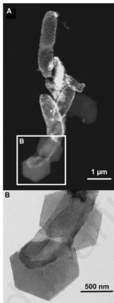
Figure 10: Scanning transmission electron microscopy (STEM) image of BoFeN1 culture suspension after 2 days measured in the high angular annular dark field mode (HAADF) (A). Magnified transmission electron microscopy image of BoFeN1 cell with hexagonal carbonate GR flakes measured in brightfield mode (B). Reproduced from Ref. 274. Copyright 2012 American Chemical Society.
