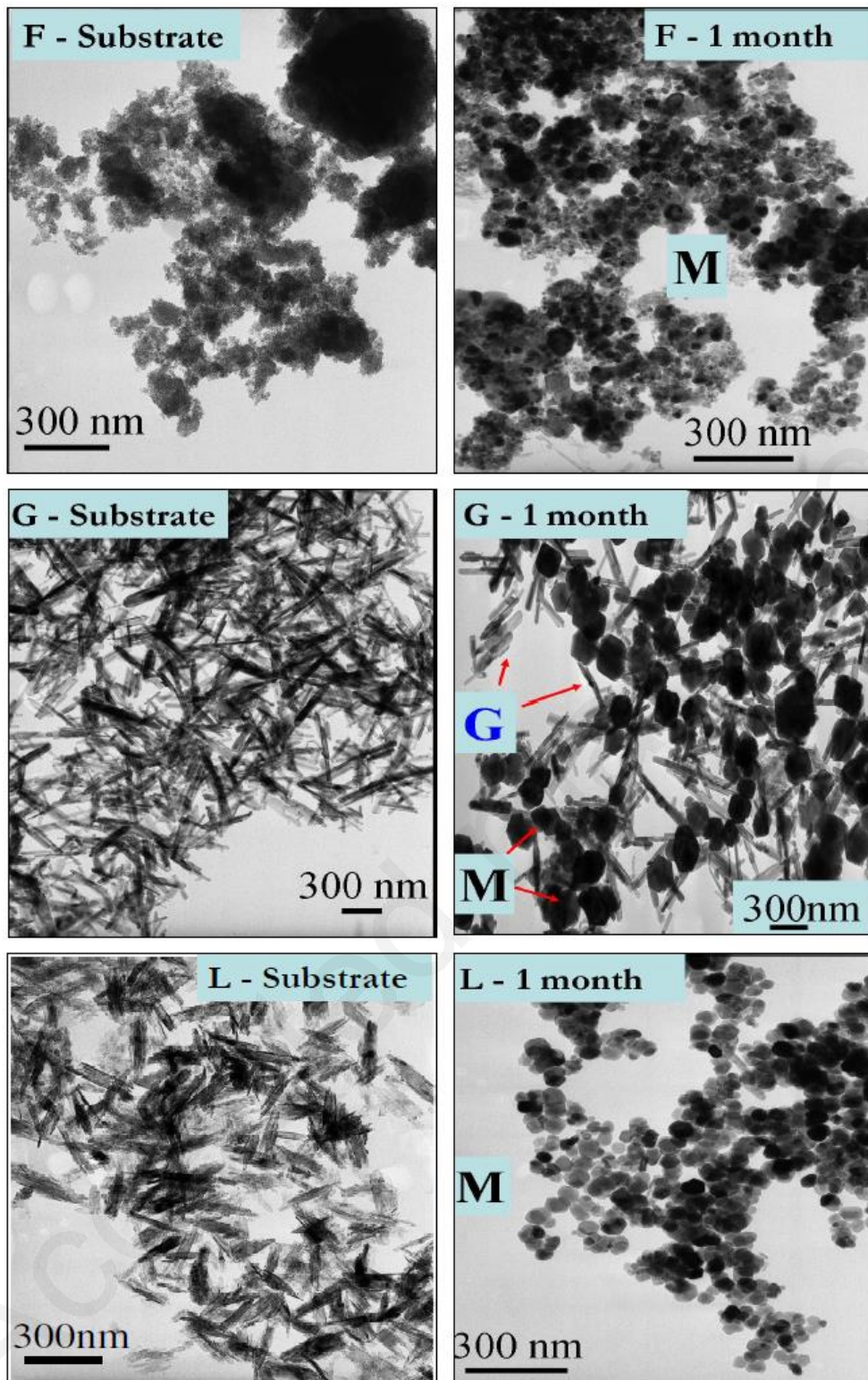
Figure 8: Bright field transmission electron microscopy images showing initial ferric (oxyhydr)oxides (ferrhydrite-F, lepidocrocite-L and goethite-G) and their transformations products after their reaction with suitable amounts of Fe(II) and \text{OH}^- to form stoichiometric magnetite (M). Transformation product of G indicates the presence of M and untransformed G. Reproduced with permission from Ref. 37. Copyright 2012 Elsevier.
