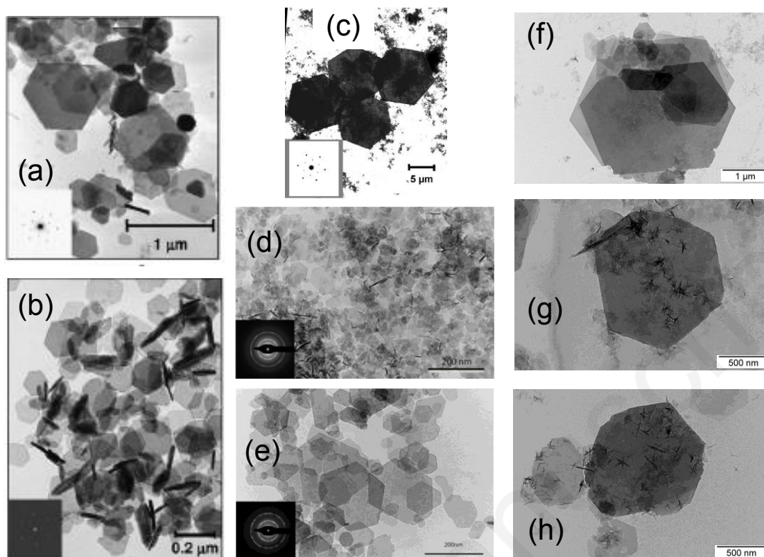
Figure 18: TEM images of different green rusts formed by different procedures. (a) \text{GR}(\text{SO}_4^{2-}) and (b) \text{GR}(\text{CO}_3^{2-}) were formed by coprecipitation. 31 Reproduced with permission from Ref. 31. Copyright 2006 Elsevier Masson SAS. (c) \text{GR}(\text{CO}_3^{2-}) formed by bioreduction of lepidocrocite. 389 Reproduced from Ref. 389. Copyrights 2002 American Chemical Society. (d) and (e) correspond to \text{GR}(\text{CO}_3^{2-}) formed by coprecipitation but samples were aged for 0 h and 24 h respectively. 390 Reproduced with permission from Ref. 390. Copyright 2012 Elsevier. (f), (g) and (h) correspond to the \text{GR}(\text{SO}_4^{2-}) formed by abiotic mineralogical transformations of ferrihydrite, goethite and hematite respectively where traces of goethite and hematite are still visible in (g) and (h), respectively. 51 Reproduced with permission from Ref. 51. Copyright 2012 Elsevier.
