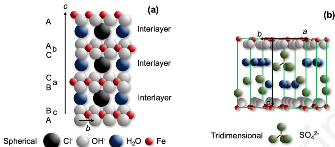
Figure 2: General view of the crystal structure of green rusts: (a) GR-I (Cl - ) (b) GR-II (SO 4 2- ). Image (a) is adapted with permission from Ref. 26. Copyright 1998 Elsevier. Image (b) is adapted with permission from Ref. 24. Copyright 2003 Elsevier Masson SAS.
