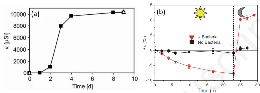
Figure 21: (a) Changes to volume-dependent magnetic susceptibility ( \kappa ) during microbial reduction of ferrihydrite to magnetite. 398 Reproduced from Ref. 398. Copyright 2010 American Chemical Society. (b) Relative changes to \kappa during the incubation of magnetite with Fe(II)-oxidizing and Fe(III)-reducing bacteria. Decreases in \kappa correspond to oxidation whilst increases in \kappa correspond to reduction. 313 Reproduced with permission from Ref. 313. Copyright 2015 The American Association for the Advancement of Science.
