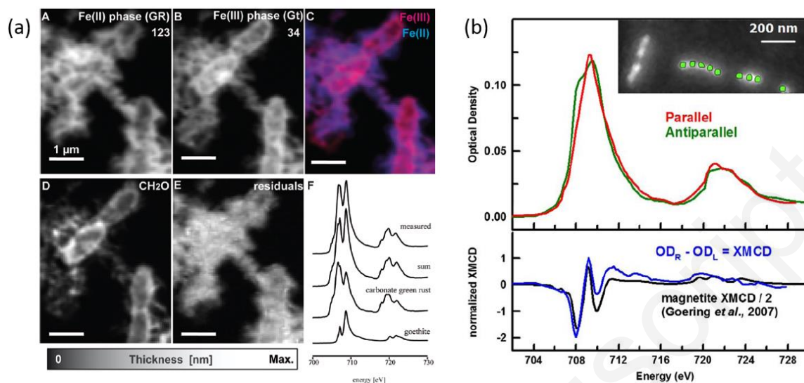
Figure 17: (a) The formation of mixed-valent green rust as an intermediate phase before goethite formation during microbial Fe(II) oxidation was shown using STXM. Reproduced from Ref. 274 . Copyright 2012 American Chemical Society. (b) STXM can be combined with XMCD to provide the cation distribution of Fe(II) and Fe(III) in individual magnetosomes formed within magnetotactic bacteria. Reproduced with permission from Ref. 281 . Copyright 2010 Elsevier.
