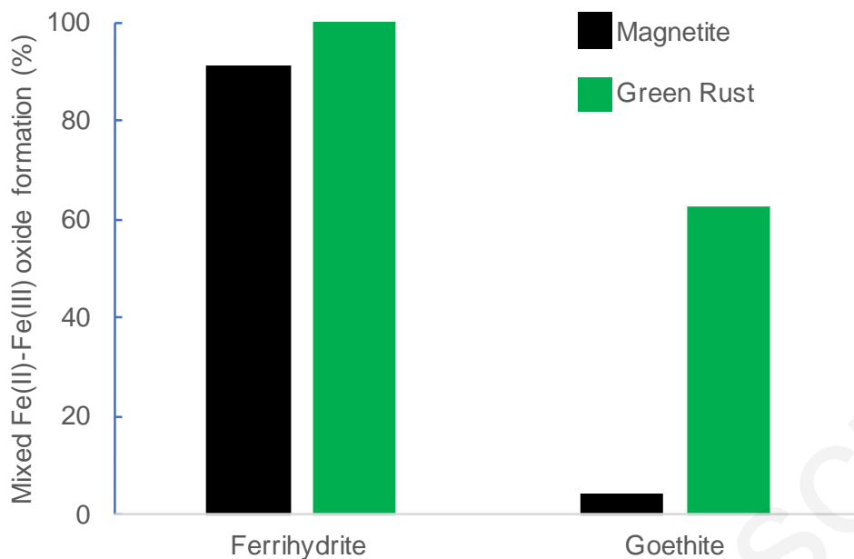
Figure 7: Transformation extent of ferrihydrite and goethite into mixed-valent iron minerals (magnetite and green rust) measured by Mössbauer Spectroscopy. Ferrihydrite and goethite were reacted with stoichiometric amounts of soluble Fe(II) and NaOH to form magnetite and green rust according to the reaction 3 and 4. Figure prepared by using the data reported in Table 2 of Ref. 51.
