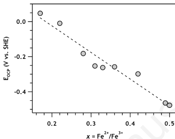
Figure 3: Open circuit potentials ( E_{\text{OCP}} ) of magnetite as a function of stoichiometry (Fe(II)/Fe(III) ratio). Reproduced from Ref. 39. Copyright 2009 American Chemical Society.
