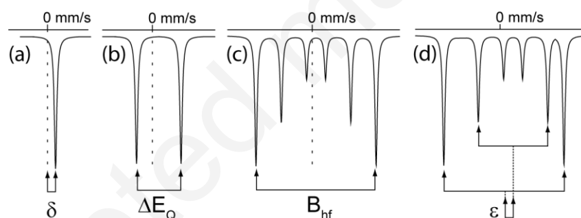
Figure 14: Mössbauer parameters, (a) isomer shift \delta , (b) quadrupole splitting \Delta E_Q , (c) magnetic hyperfine field B_{hf} , (d) quadrupole shift \epsilon .
