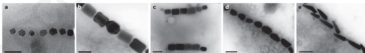
Figure 11: Different morphologies of magnetite produced by MTB's. Reproduced with permission from Ref. 294. Copyright 2016 Nature Publishing Group.
