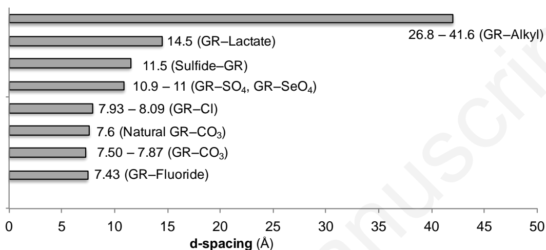
Figure 13: Variation of d -spacings in XRD parameters of different GRs depending upon their type and nature of intercalated molecules. This figure is based on the data compiled in previous studies 22,26,88,331,332 and references cited therein.
