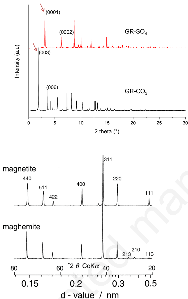
Figure 12. X-ray diffractograms of green rusts namely GR(SO 4 2- ) and GR(CO 3 2- ), magnetite, and maghemite. Diffractograms of GR(SO 4 2- ) and GR(CO 3 2- ) are reproduced with permission from Ref. 19. Copyright 2010 Elsevier. Diffractograms of magnetite and maghemite are reproduced with permission from Ref. 2. Copyright 2003 Wiley-VCH Verlag GmbH & Co. KGaA.
