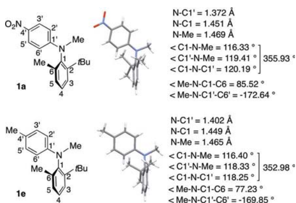
Figure 5. X-Ray crystal structures of 1a and 1e.
