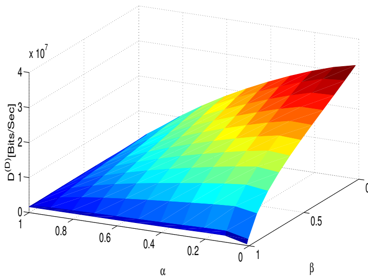
Fig. 11. DVB data rate w.r.t. \alpha and \beta when IAPA is applied, d = 1000 m.
