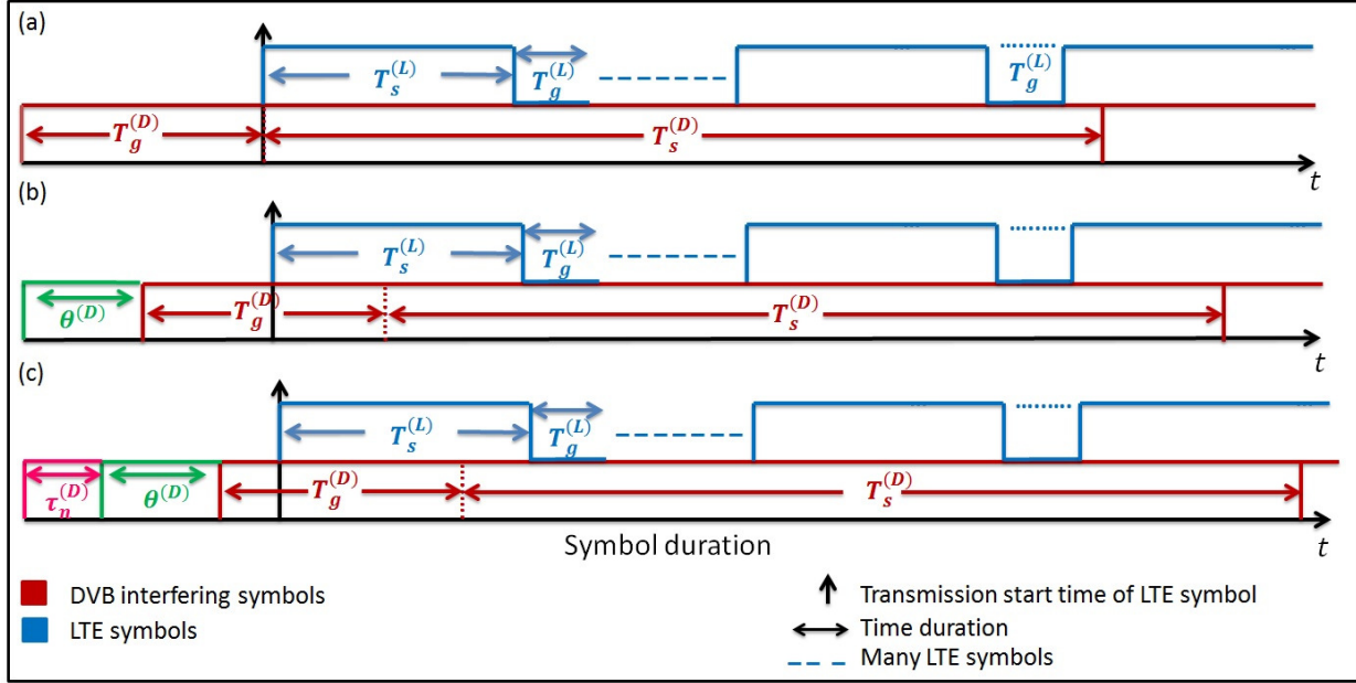
Fig. 3. Interfering DVB symbols over LTE symbol
