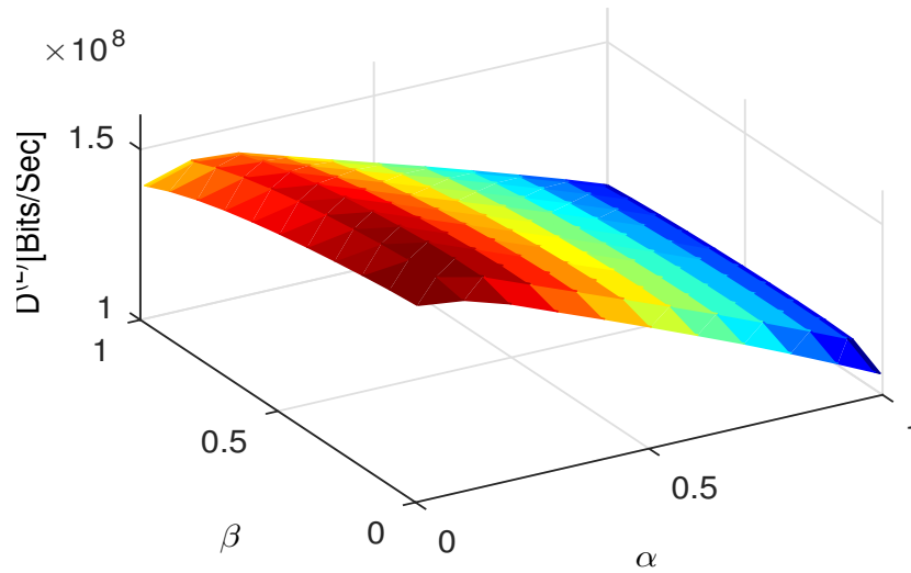
Fig. 12. LTE data rate w.r.t. \alpha and \beta when IAPA is applied, d = 1000 m.
