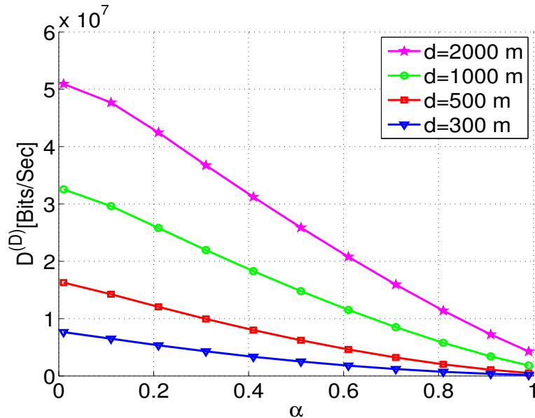
Fig. 6. DVB data rate in [Bits/sec] w.r.t. \alpha and labeled on d=300, 500, 1000 m when UPA is applied
