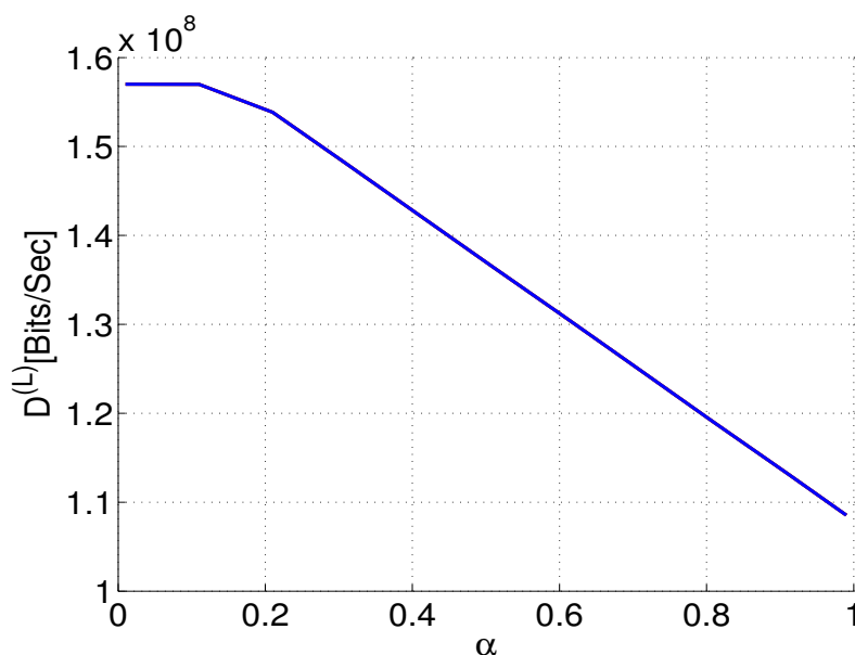
Fig. 5. LTE data rate in [Bits/sec] w.r.t. \alpha when UPA is applied.
