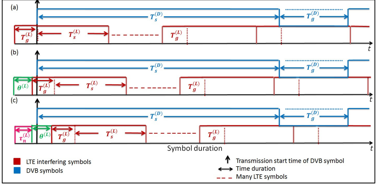
Fig. 4. Interfering LTE symbols over DVB symbol
