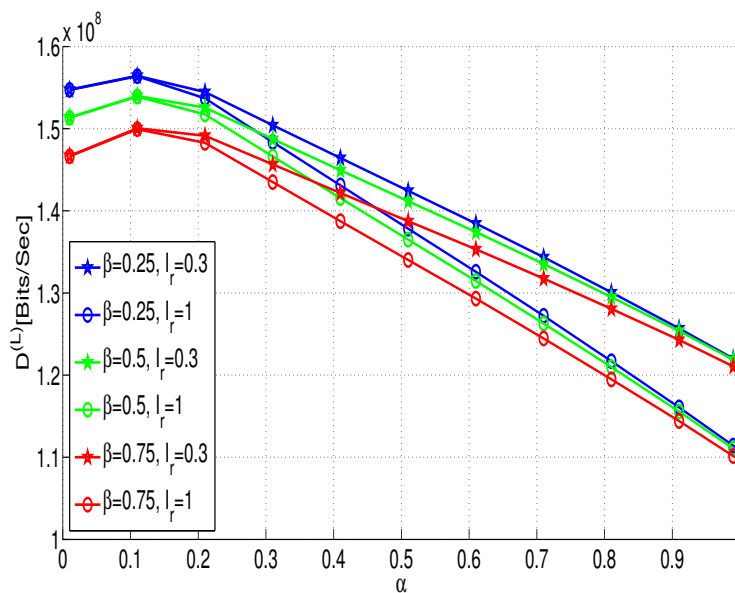
Fig. 8. LTE data rate w.r.t. \alpha labeled on interference cancellation coefficient and IAPA parameter \beta and d = 1000 m.
