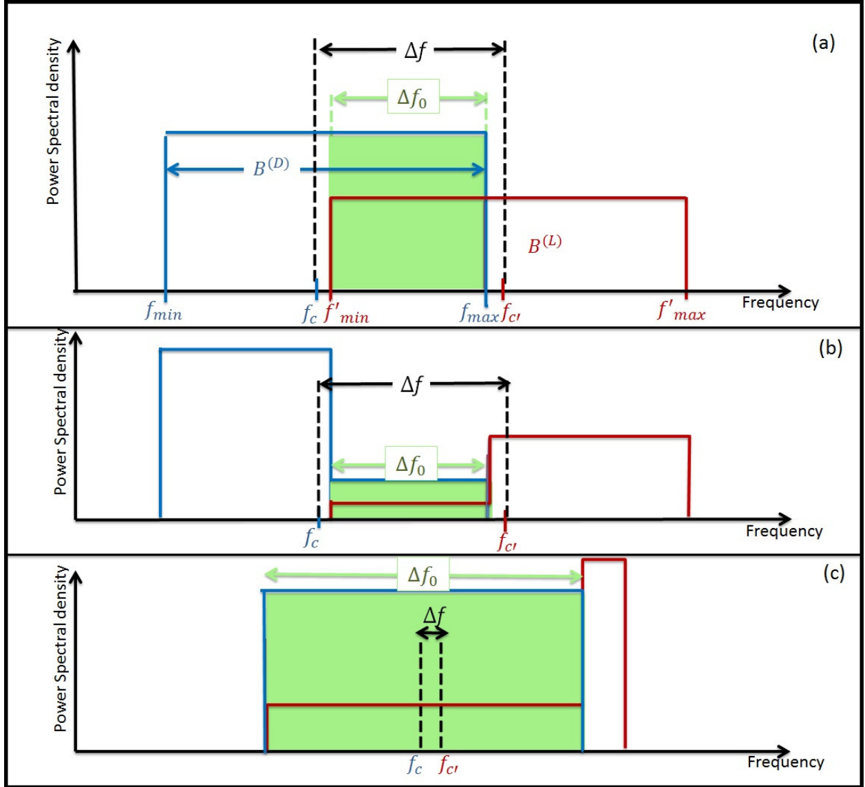
Fig. 2. Spectral overlap presentation
