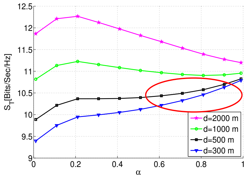
Fig. 7. Global spectral efficiency w.r.t. \alpha and labeled on d=300, 500, 1000 m when UPA is applied.
