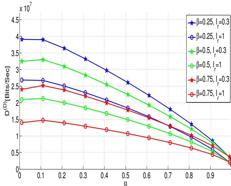
Fig. 9. DVB data rate w.r.t. \alpha labeled on interference-cancellation coefficient and IAPA parameter \beta and d = 1000 m.
