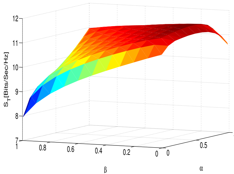
Fig. 13. Global spectral efficiency w.r.t. \alpha and \beta when IAPA is applied, d = 1000 m.
