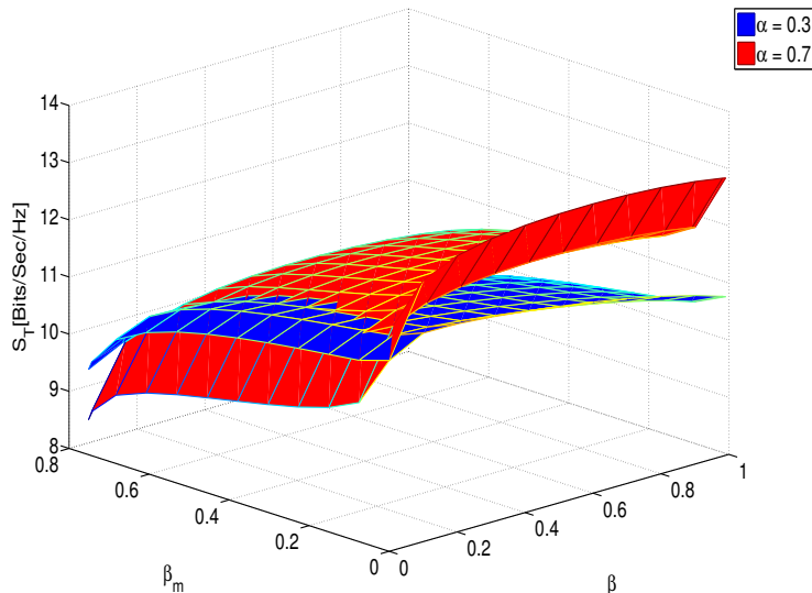
Fig. 16. Global spectral efficiency w.r.t. \beta and \beta_m when IAPA is applied, d = 1000 m, for \alpha = 0.3 and \alpha = 0.7 .
