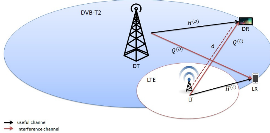
Fig. 1. System model: DVB-LTE coexistence
