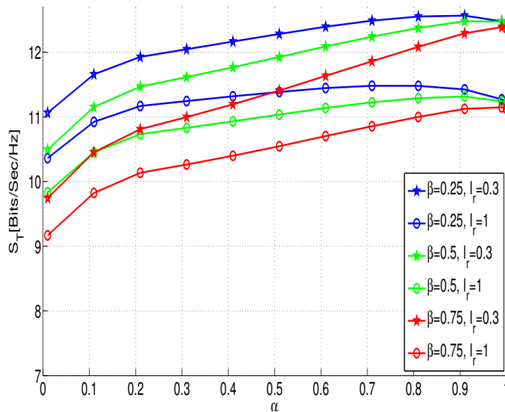
Fig. 10. Global spectral efficiency w.r.t. \alpha labeled on interference-cancellation coefficient and IAPA coefficient \beta and d = 1000 m.
