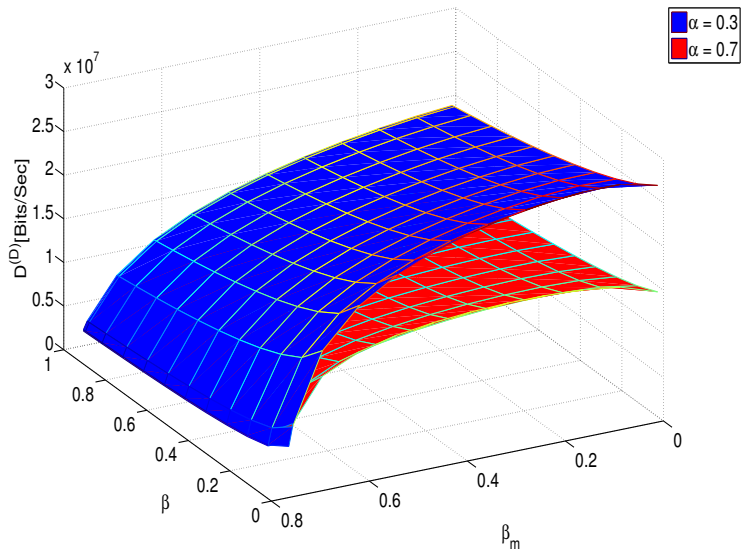
Fig. 14. DVB data rate w.r.t. \beta and \beta_m when IAPA is applied, d = 1000 m, for \alpha = 0.3 and \alpha = 0.7 .
