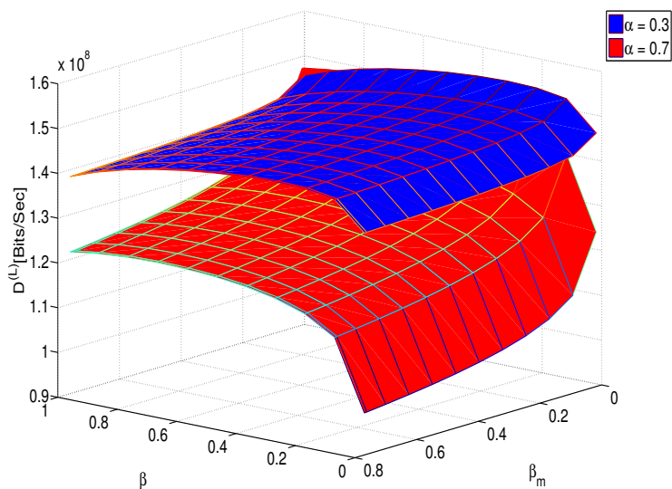
Fig. 15. LTE data rate w.r.t. \beta and \beta_m when IAPA is applied, d = 1000 m, for \alpha = 0.3 and \alpha = 0.7 .
