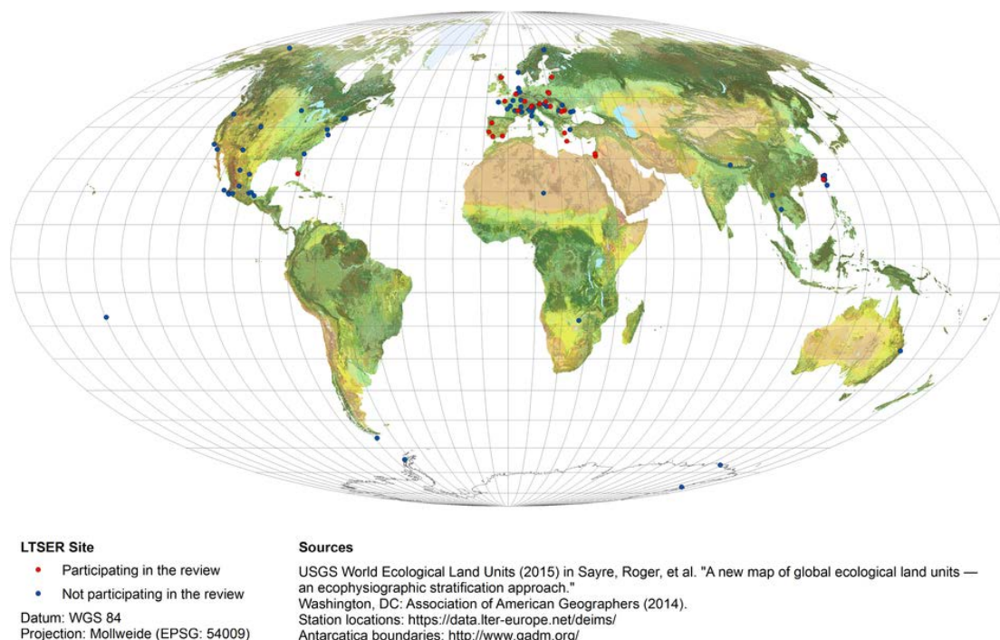
Figure 1 LTSER platforms identified in the DEIMS-SDR metadata search and annotated according to those participating and those not participating in this review.
