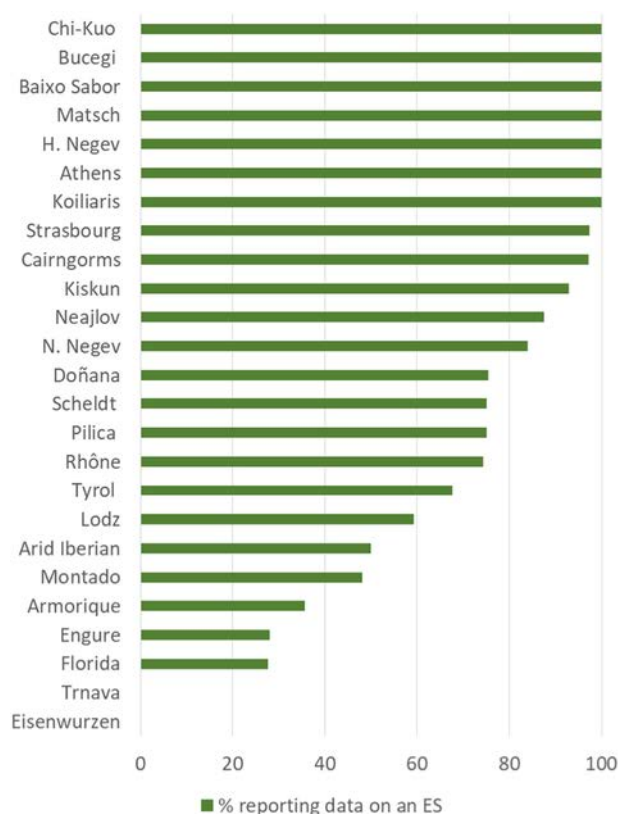
Figure 6 Proportion of publications reviewed (n = 1,112) which reported on at least one ecosystem service (see Table 1 for explanation of the platform codes and number of papers reviewed).
