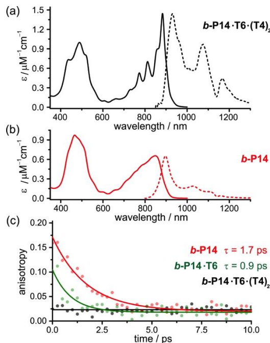
Figure 4. UV-vis-NIR absorption (solid line) and fluorescence (dashed line) spectra of (a) b -P14·T6·(T4) 2 and (b) b -P14 (toluene, 298 K). The dip at 1130–1170 nm corresponds to solvent absorption. (c) First order fits of the fluorescence anisotropy decay. Solutions of b -P14·T6·(T4) 2 (black), b -P14·T6 (green) and b -P14 (red) were excited at 820 nm and emission was detected at 950 nm.
