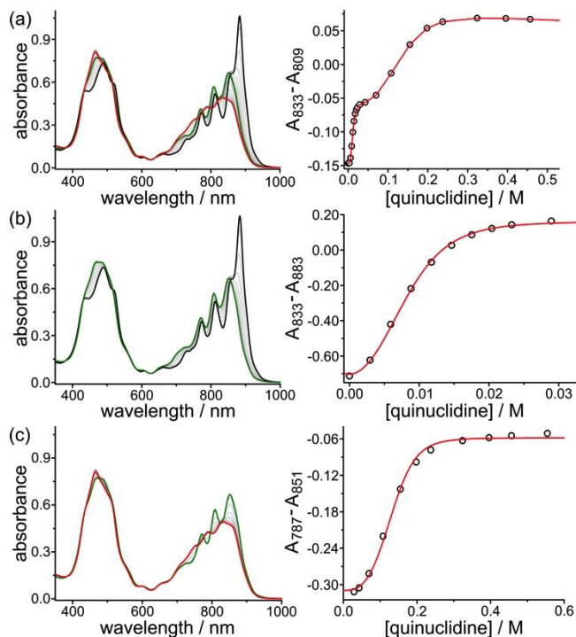
Figure 3. UV-vis-NIR denaturation titration of the b -P14·T6·(T4) 2 complex with quinuclidine (toluene, 298 K). (a) Full titration, T4 is displaced first (black to green) followed by the displacement of T6 (green to red). The two phases of the titration are shown in (b) and (c), with the experimental (black circles) and calculated isotherms (red lines) shown on the right.
