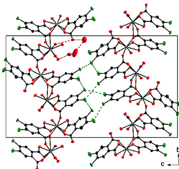
Figure 4. Projection view of an extended unit cell of [\text{Er}_2(\text{dcpa})_3(\text{H}_2\text{O})_5 \cdot 3\text{H}_2\text{O}]_\infty . Hydrogen bonds and halogen bonds are symbolized by red and green broken lines respectively.
