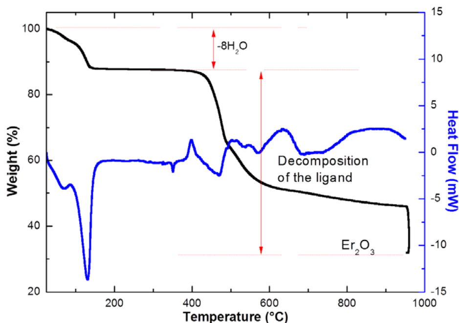
Figure 5. TGA/DSC of [\text{Er}_2(\text{dcpa})_3(\text{H}_2\text{O})_5 \cdot 3\text{H}_2\text{O}]_\infty between room temperature and 950 °C under nitrogen atmosphere. At 950 °C, nitrogen is replaced by air in order to insure complete decomposition.
