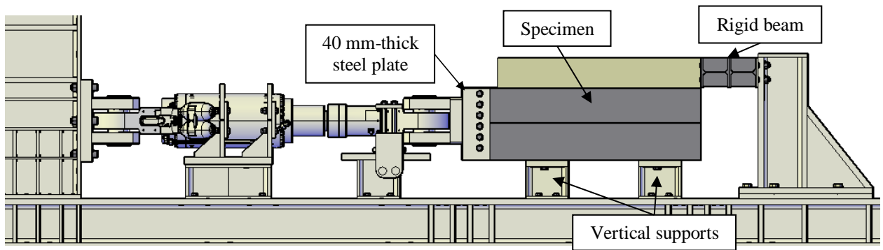
Figure 2: Schematic of push-out test setup.
