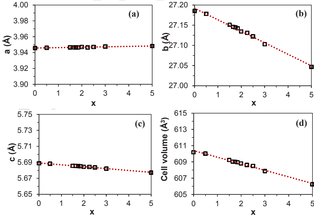
Figure 2. Evolution as a function of the composition ( x ) of: (a)(b)(c) cell parameters and (d) cell volume of (Sr_2Ta_2O_7)_{100-x}(La_2Ti_2O_7)_x powders synthesized by solid state route (the uncertainty on each value is always less than the height of the drawn symbol).
