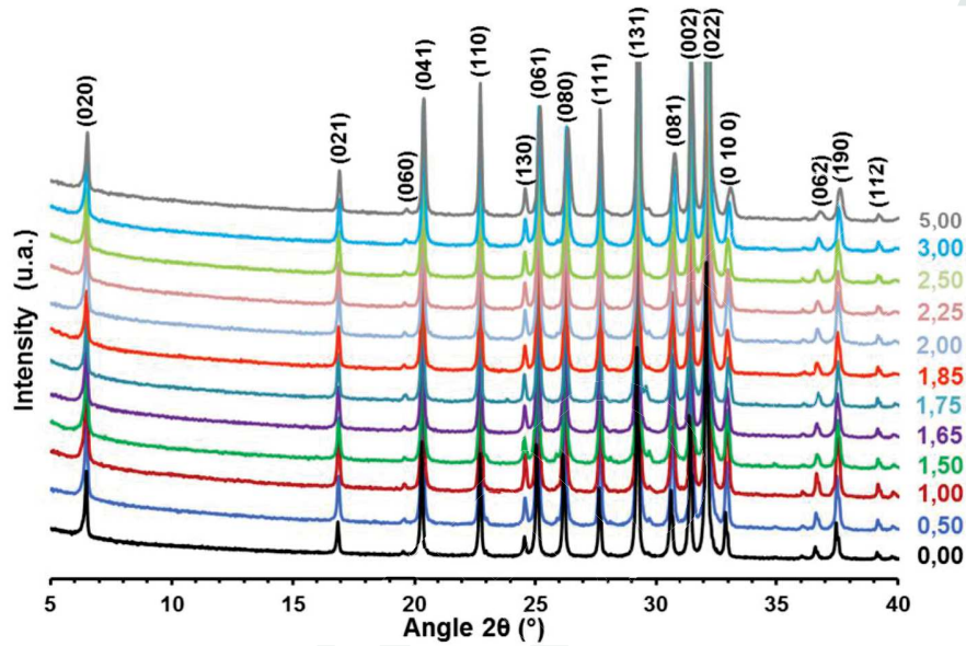
Figure 1. \theta - 2\theta X-ray diagrams of the (Sr_2Ta_2O_7)_{100-x}(La_2Ti_2O_7)_x powders with 0 \leq x \leq 5 , synthesized by solid state route. Diffraction peaks are indexed according to an isotype of the paraelectric Sr_2Ta_2O_7 compound (JCPDS File No.70-0248).
