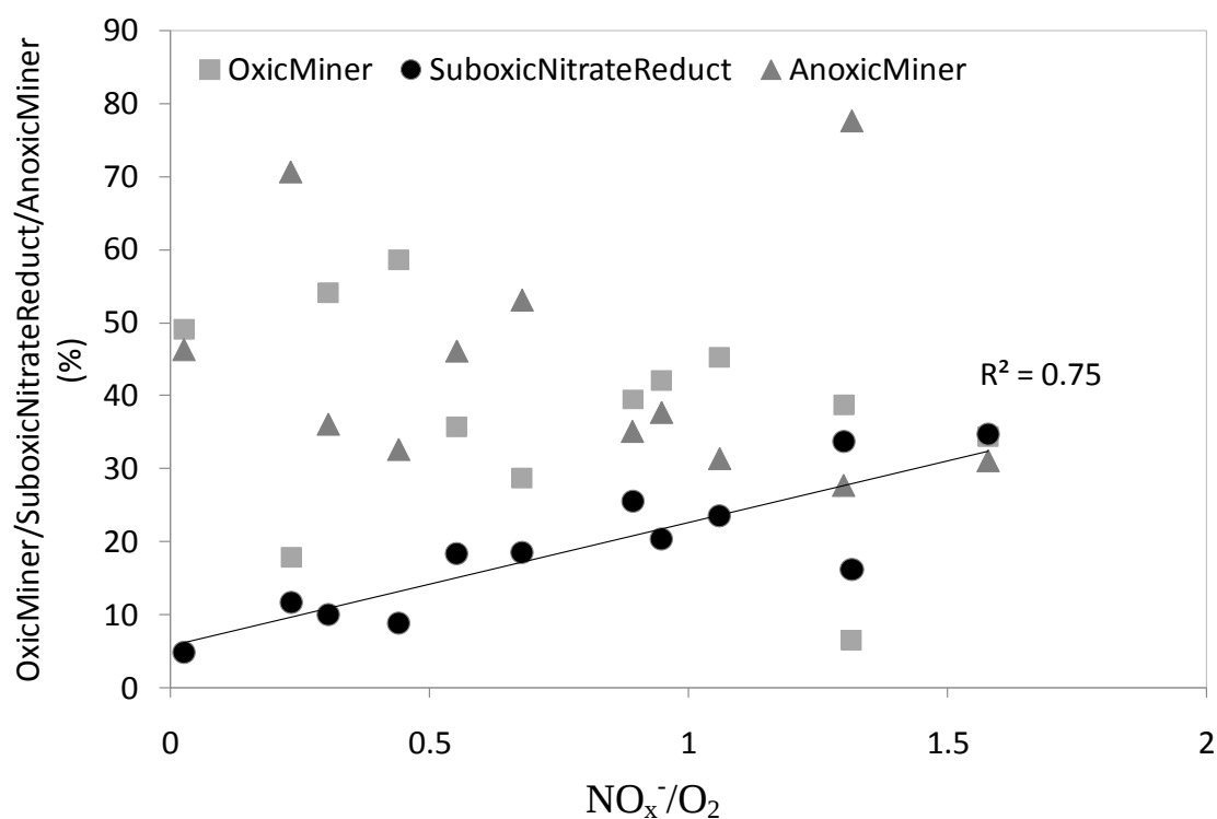
Fig. 6 Variation of oxic mineralization (%), suboxic nitrate reduction (%) and anoxic mineralization (%) with \text{NO}_x:\text{O}_2 ratio, at Elorn and Aulne stations in two seasons. Clear linear correlation between suboxic nitrate reduction (%) and \text{NO}_x:\text{O}_2 ratio is found with R^2 = 0.75 .
