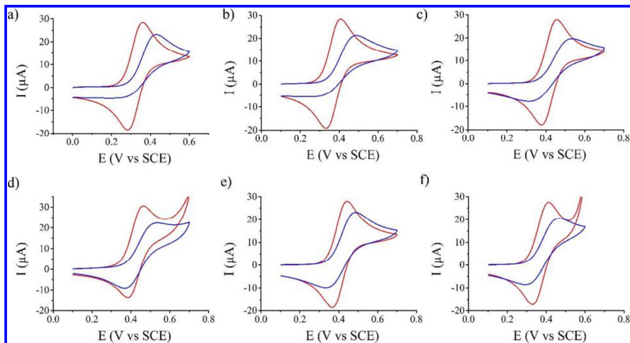
Figure 7. Cyclic voltammetry of 10^{-3} mol L ^{-1} of ferrocene in acetonitrile solution containing a) 0.1 mol L ^{-1} potassium hexafluorophosphate ( \text{KPF}_6 ), b) 0.1 mol L ^{-1} tetraethylammonium hexafluorophosphate ( \text{Et}_4\text{NPF}_6 ), c) 0.1 mol L ^{-1} tetraoctylammonium hexafluorophosphate ( n\text{Oc}_4\text{NPF}_6 ), d) 0.1 mol L ^{-1} tetrabutylammonium chloride ( n\text{Bu}_4\text{NCl} ), e) 0.1 mol L ^{-1} tetrabutylammonium tetrafluoroborate ( n\text{Bu}_4\text{NBF}_4 ) and f) 0.1 mol L ^{-1} tetrabutylammonium tetraphenylborate ( n\text{Bu}_4\text{NBPh}_4 ), on bare carbon electrodes (red curves) and on carbon electrodes modified by thick organic films (blues curves). Scan rate: 100 mV s ^{-1} .
