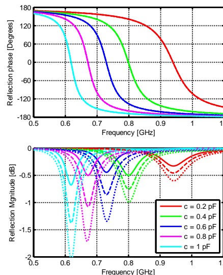
Fig. 3. Simulated AMC unit cell reflection phase (top) and magnitude (bottom) for various tuning capacitance values and various ohmic resistance values (Solid line, R=0.1 Ohm, Dashed line, R=1 Ohm. Dotted line, R=2 Ohm)
