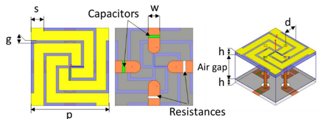
Fig. 1. Unit-cell geometry of the proposed AMC (left: top view, center: bottom view and right: perspective view)
