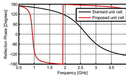
Fig. 2. Simulated reflection coefficient phase of the proposed AMC compared to with a conventional mushroom-like unit cell.
