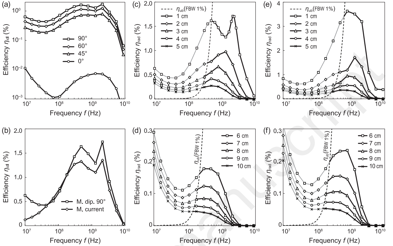
FIG. 3. Radiation efficiencies \eta_{idl} and \eta_{rad} in infinite planar-bounded media. (a) Orientation of the magnetic dipole moment \mathbf{m} strongly affects the efficiency (homogeneous half-space). (b) The 90^\circ -oriented magnetic dipole moment \mathbf{m} ( TM_z mode) compared to the out-of-plane magnetic current source ( TE_z mode) at d = 1 cm in the homogeneous half-space medium. (c) The homogeneous half-space medium at d = 1 to 5 cm and (d) at d = 6 to 10 cm implantation depths. (e) The layered (skin-fat-muscle) half-space medium at d = 1 to 5 cm and (f) at d = 6 to 10 cm implantation depths.
