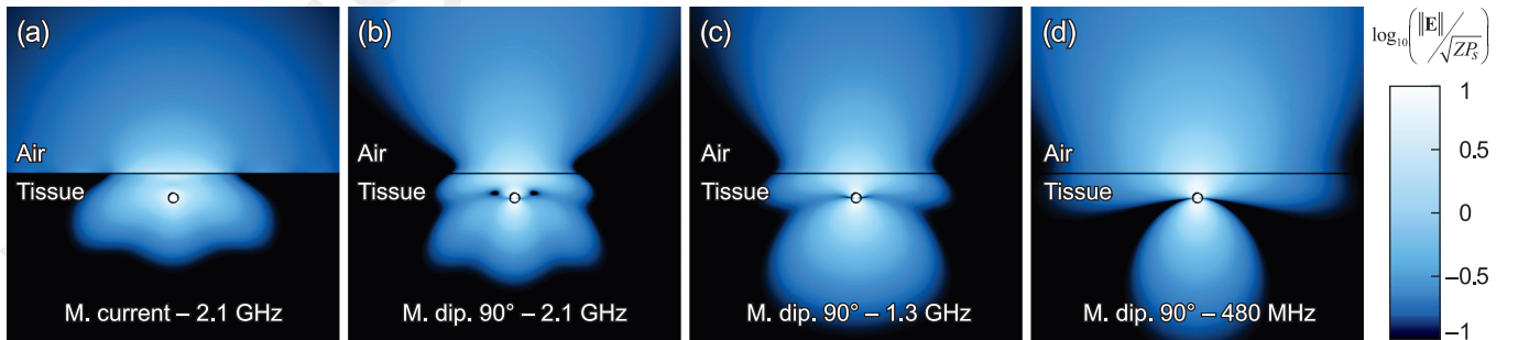
FIG. 4. Normalized \mathbf{E} -field distributions at d = 1 cm in infinite planar-bounded homogeneous half-space media. (a) The magnetic current source ( TE_z mode) and (b)–(c)–(d) The 90^\circ -oriented magnetic dipole ( TM_z mode). The radiation efficiency peaks at 2.1 GHz (a)–(b) and 480 MHz (d) for both sources and drops at 1.3 GHz (c) due to the interference with reflected wave.
