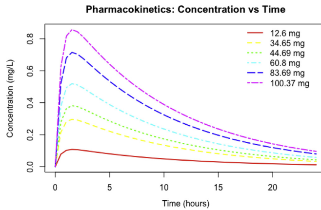
Fig. 3. Plot of the concentration of the drug vs time for 12.6, 34.65, 44.69, 60.8, 83.69 and 100.37 mg with k_a = 2h^{-1} , CL = 10Lh^{-1} and V = 100L .
