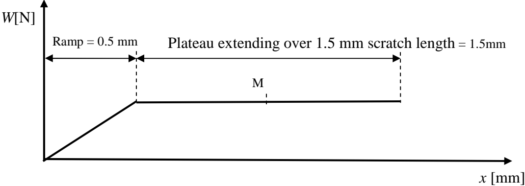
Fig. 2: Loading path consisting of a ramp and a constant-load plateau
