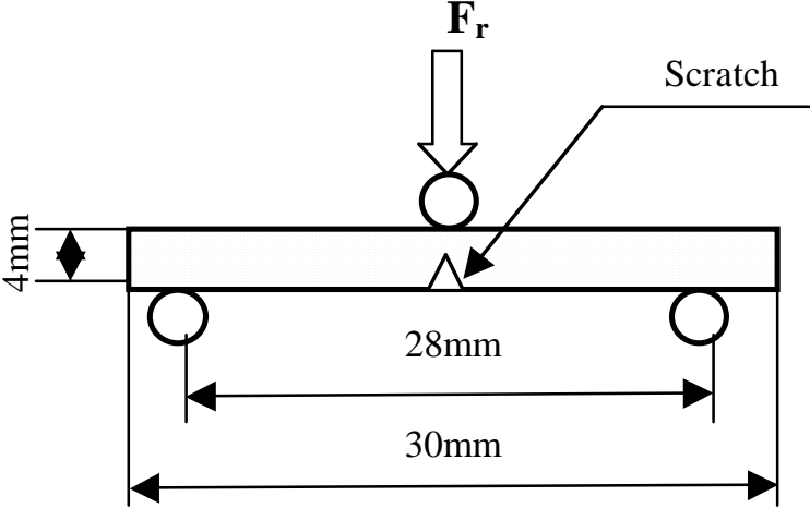
Fig. 3: Three-points bending test.
