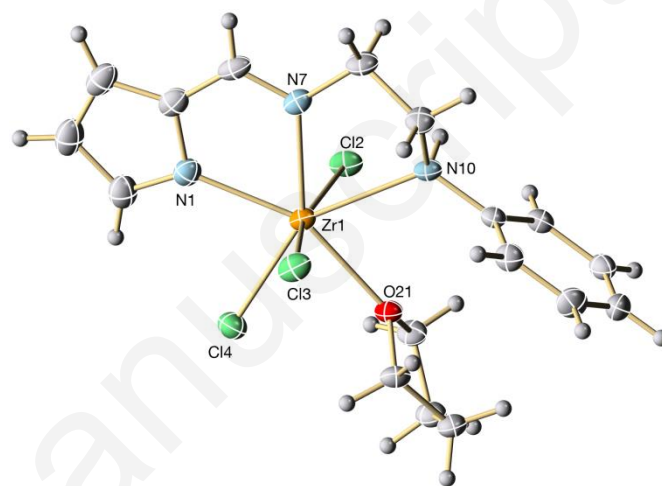
Fig. 1 ORTEP drawing of [\text{Zr}\{2-(\text{C}_4\text{H}_3\text{N}-2\text{-CH}=\text{N})\text{C}_2\text{H}_4\text{NHPh}\}(\text{THF})\text{Cl}_3] ( 2a ) (thermal ellipsoids drawn at the 30% probability level). Selected bond distances (Å) and angles (deg): \text{Zr}(1)-\text{N}(1) = 2.251(2) , \text{Zr}(1)-\text{O}(21) = 2.2985(16) , \text{Zr}(1)-\text{N}(7) = 2.3221(19) , \text{Zr}(1)-\text{Cl}(2) = 2.4318(6) , \text{Zr}(1)-\text{Cl}(3) = 2.4291(6) , \text{Zr}(1)-\text{Cl}(4) = 2.4987(7) , \text{Zr}(1)-\text{N}(10) = 2.526(2) . \text{N}(1)-\text{Zr}(1)-\text{O}(21) = 151.10(7) , \text{N}(1)-\text{Zr}(1)-\text{N}(10) = 135.52(7) , \text{N}(1)-\text{Zr}(1)-\text{N}(7) = 70.04(7) , \text{N}(7)-\text{Zr}(1)-\text{N}(10) = 66.02(7) , \text{O}(21)-\text{Zr}(1)-\text{N}(7) = 138.82(7) , \text{N}(1)-\text{Zr}(1)-\text{Cl}(3) = 98.97(5) , \text{O}(21)-\text{Zr}(1)-\text{Cl}(3) = 87.07(4) , \text{N}(7)-\text{Zr}(1)-\text{Cl}(3) = 85.97(5) , \text{N}(1)-\text{Zr}(1)-\text{Cl}(2) = 93.91(5) , \text{O}(21)-\text{Zr}(1)-\text{Cl}(2) = 86.19(4) , \text{N}(7)-\text{Zr}(1)-\text{Cl}(2) = 89.58(5) , \text{Cl}(3)-\text{Zr}(1)-\text{Cl}(2) = 164.0(2) , \text{N}(1)-\text{Zr}(1)-\text{Cl}(4) = 77.61(6) , \text{O}(21)-\text{Zr}(1)-\text{Cl}(4) = 73.79(4) , \text{N}(7)-\text{Zr}(1)-\text{Cl}(4) = 147.18(5) , \text{Cl}(3)-\text{Zr}(1)-\text{Cl}(4) = 93.8(2) , \text{Cl}(2)-\text{Zr}(1)-\text{Cl}(4) = 98.14(2) , \text{O}21-\text{Zr}1-\text{N}10 = 72.95(6) , \text{Cl}(3)-\text{Zr}(1)-\text{N}(10) = 84.69(5) , \text{Cl}(2)-\text{Zr}(1)-\text{N}(10) = 79.46(5) , \text{Cl}(4)-\text{Zr}(1)-\text{N}(10) = 146.73(5) .
