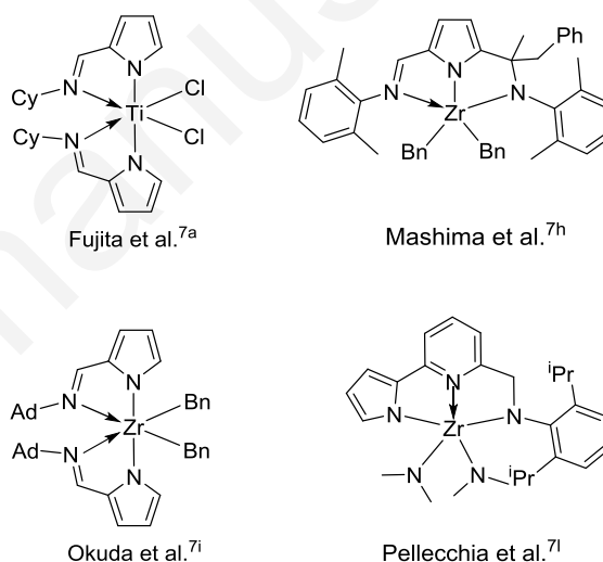
Chart 1. Selected examples of Group 4 complexes supported by pyrrolyl-based ligands applied in homopolymerization of ethylene.
