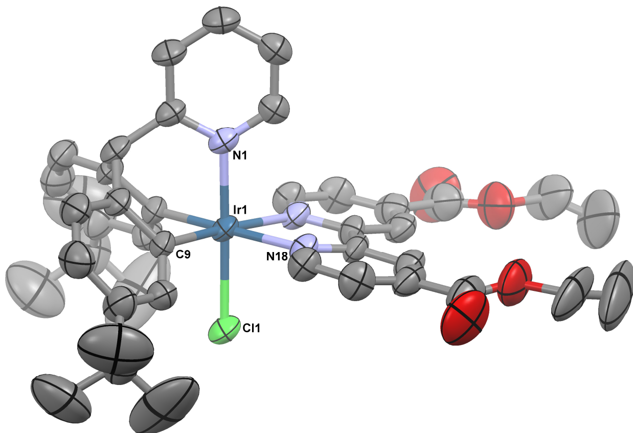
Figure 1. Solid-state structure of complex 1, thermal ellipsoids are drawn at the 50 % probability level. Hydrogen atoms and solvent molecules are omitted for clarity (color code: C = grey, N = purple, O = red, Cl = green and Ir = blue).
