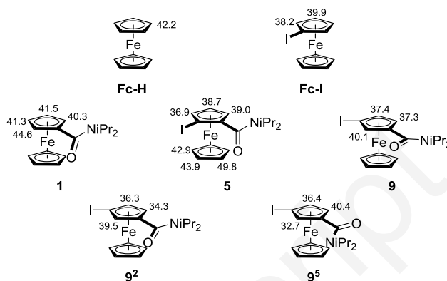
Chart 3. Selected calculated \text{pK}_a values in THF solution for 5·LiF (most stable conformation of 5 ) and 9·LiF ( \text{Cp} and \text{C}=\text{O} coplanar).
