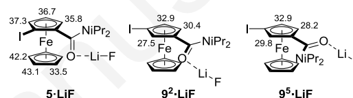
Chart 3. Selected calculated \text{pK}_a values in THF solution for 5·LiF (most stable conformation of 5 ) and 9·LiF ( \text{Cp} and \text{C}=\text{O} coplanar).
