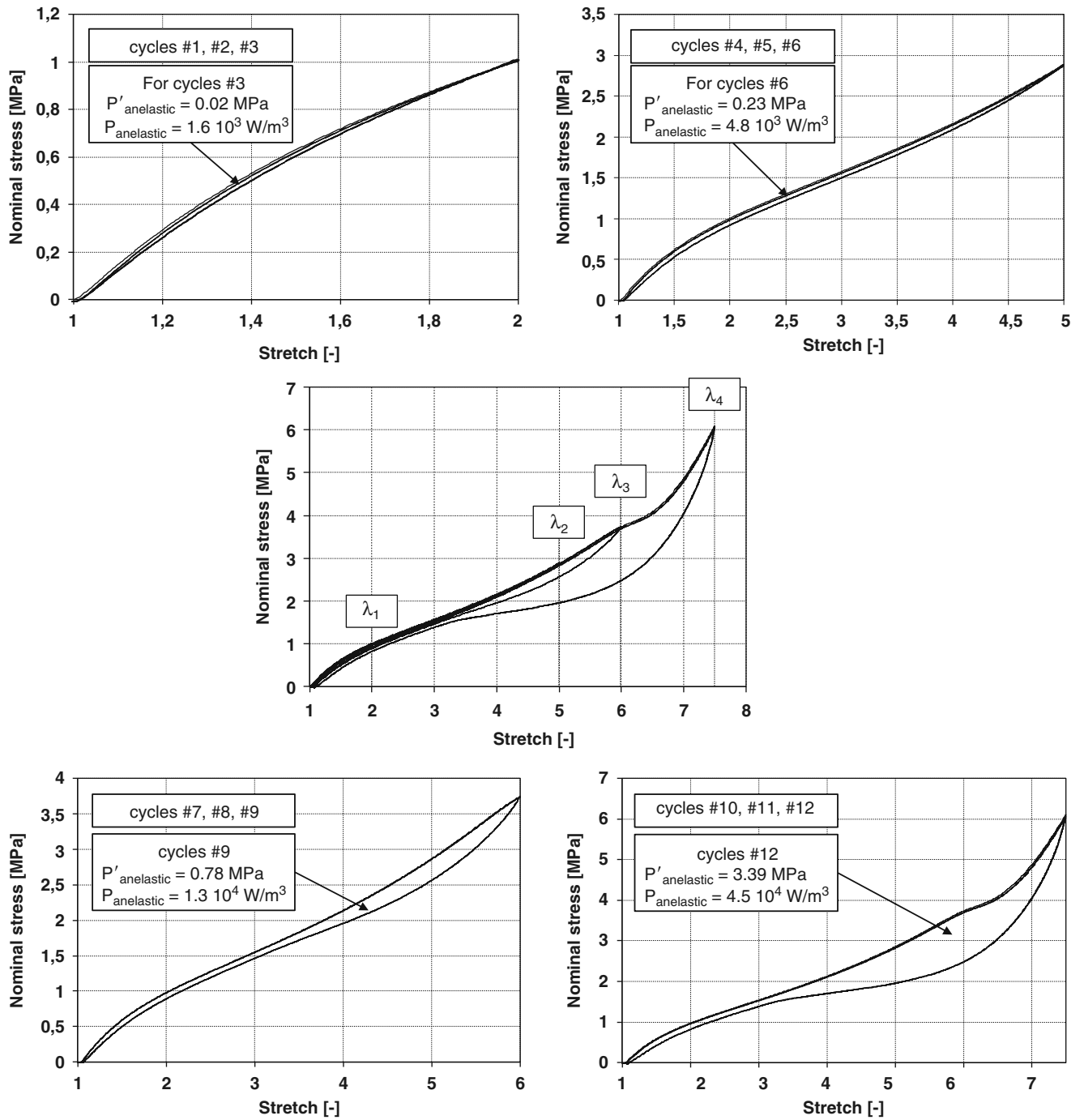
Fig. 6.1 Mechanical response
